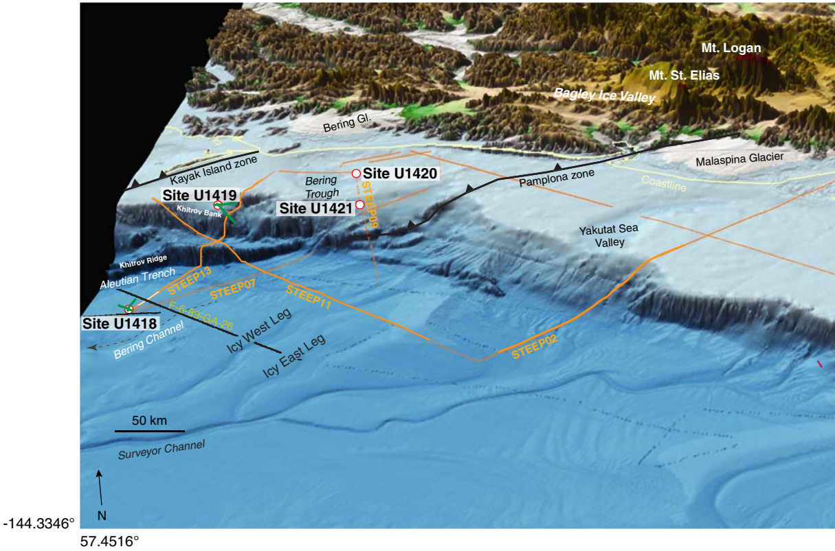
Figure F38. Perspective view of the northern Gulf of Alaska showing major tectonic elements with thrust faults in black. Relief is shown at ~10× vertical exaggeration, with total vertical relief displayed ranging from <4000 m below sea level to >5000 m above sea level. Black = U.S. Geological Survey, green = Cruise EW0408, orange = seismic profiles from St. Elias Erosion/Tectonics Project (STEEP), draped over topography. Figure is modified from Gulick et al. (2013).
