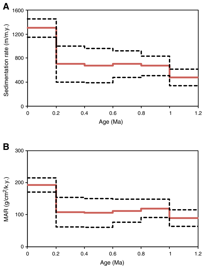
Figure F45. (A) Shipboard sedimentation rate and (B) mass accumulation rates (MAR) for Site U1418, based on the CCSF-B depth model, the shipboard age models, and interval-averaged discrete dry density data. Values are calculated over 0.2 m.y. intervals from 0 to 1.2 Ma. Solid lines = averages within each interval, dashed lines = uncertainty bounds (minimum and maximum rates based on shipboard age models).
