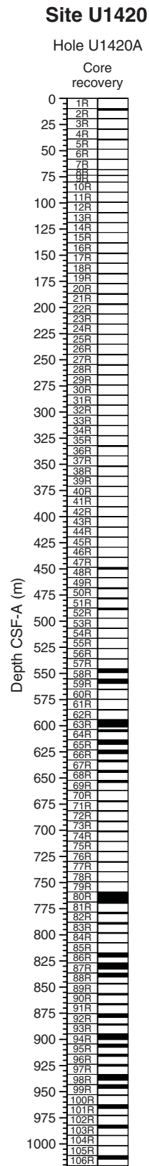
Figure F58. Core recovery, Site U1420. This consisted of a single deep borehole (U1420A).
