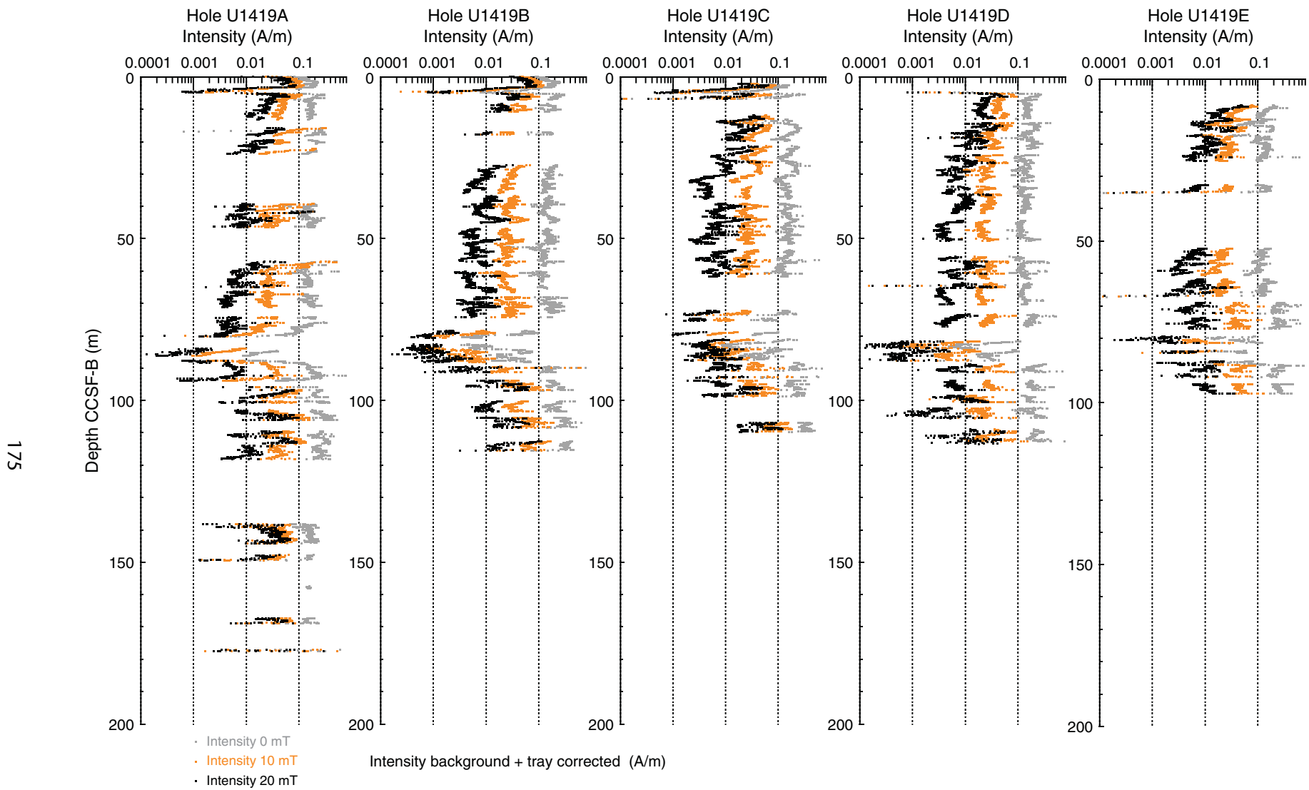
Figure F53. NRM intensities measured before and after 10 and 20 mT peak AF demagnetization, Holes U1419A–U1419E.
