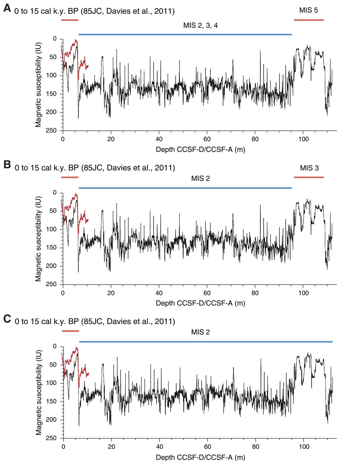
Figure F54. Preliminary shipboard chronostratigraphy, Site U1419. Based on shipboard data, three hypotheses (see text for details) were formulated; they highlight the interest of the low magnetic susceptibility interval from 96.3 to 108.2 m CCSF-A (79.1 to 87.7 m CCSF-B) for a detailed multi-proxy analysis. 85JC = site survey Core EW0408-85JC (Davies et al., 2011). Magnetic susceptibility data in red is from Davies et al. (2011). MIS = marine isotope stage. A. Hypothesis A. B. Hypothesis B. C. Hypothesis C.
