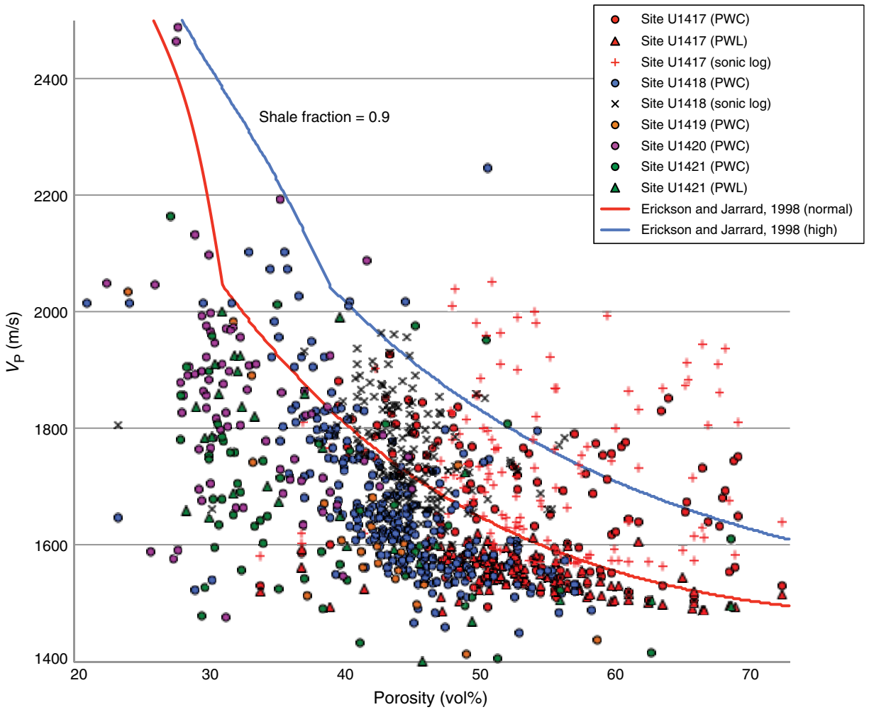
Figure F23. Expedition 341 velocity-porosity summary. PWC = P -wave caliper, PWL = P -wave logger.
