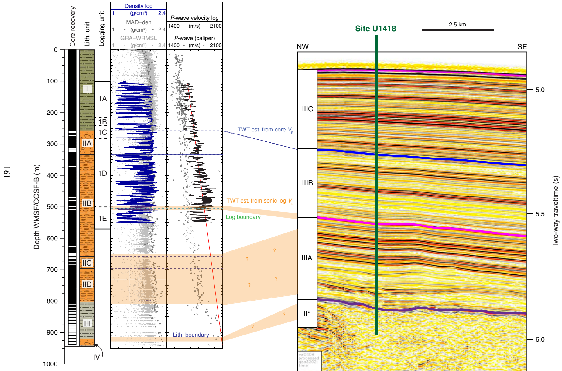
Figure F39. Comparison of sonic and density logs with discrete physical properties measurements and seismic reflection Profile GOA3202, Site U1418. Lithostratigraphic units (CCSF-B), logging units (WMSF), and seismic sequences (two-way traveltime) are shown.
