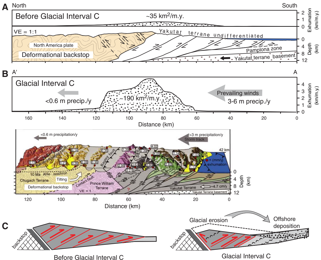
Figure F5. Proposed model of climate-related influences on orogen kinematics. Straight dashed lines depict structures with minor amounts of slip, and wavy dashed lines depict inactive structures. Strata along windward site: gray = Kultheith, green = Poul Creek, and brown = Yakataga Formations. A. Exhumational flux based on thermochronometry and architecture of the orogen prior to onset of Glacial Interval C at ~1 Ma, drawn along line A–A' (Fig. F3) based on thermochronometry (Berger et al., 2008b; Spotila and Berger, 2010) and geologic data (Plafker et al., 1994; Bruhn et al., 2004). B. Exhumational flux based on thermochronometry and architecture of the orogen after the onset of Glacial Interval C. VE = vertical exaggeration. CSEF = Chugach-St. Elias Fault, KF = Kosakuts Fault, HCF = Hope Creek Fault, MCT = Miller Creek thrust fault, SF = Sullivan Fault, AHe = apatite (U-Th)/He. D. Interpretative model of the effect of glacial erosion and deposition on the St. Elias critical wedge. Before Glacial Interval C (left), the critical Coulomb wedge is wider and has greater relief. After the intensification of glaciation (right), increased glacial erosion and offshore deposition reduced relief, concentrated deformation, required enhanced back thrusting, and forced the termination of foreland structures, thereby narrowing the wedge. Modified from Berger et al. (2008a, 2008b).
