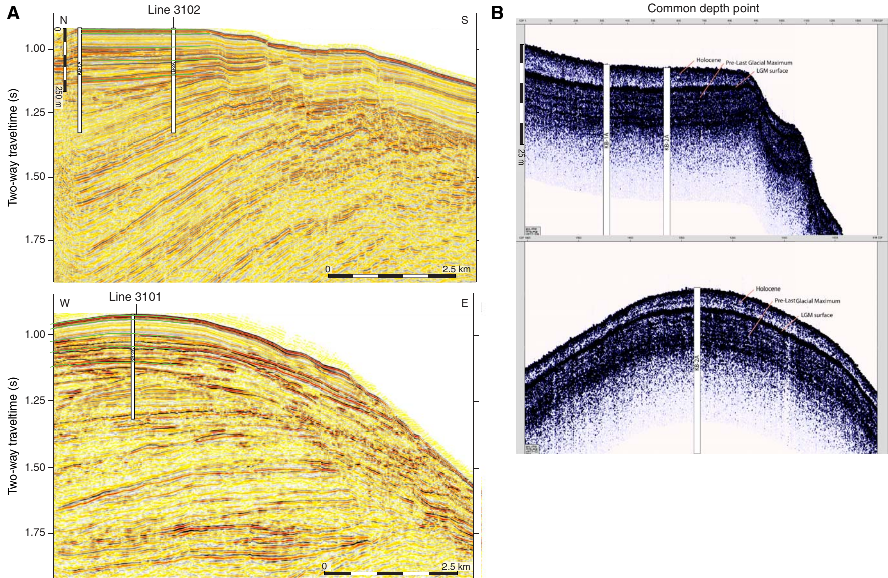
Figure F13. High-resolution seismic profiles (A) GOA-3101 and GOA-3102 and (B) CHIRP imaging the shelf break at Khitrov Ridge. Active deformation and faulting at seafloor soles into a transtensional flower structure and the drill Site KB-2 is located upslope of these structures. Higher amplitude reflectors correspond in Core EW0408 85JC (located at the landward end of seismic Profile GOA3101) to diamict (Davies et al., 2011). LGM = Last Glacial Maximum.
