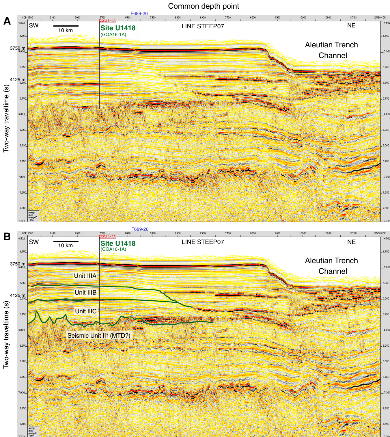
Figure F25. (A) Uninterpreted and (B) interpreted STEEP07 seismic section showing seismic facies of Sequence III on the proximal Surveyor Fan and buried mass transport deposit (MTD; Reece et al., 2012). Proposed drill sites for the proximal fan penetrate all of Sequence III and bottom in a proposed MTD (Surveyor Slide). This line is oblique to Line F-6-89-Line26 and reveals a portion of the abandoned “Bering Channel” and erosion within the Aleutian Trench Channel. Modified from Reece et al., 2012.
