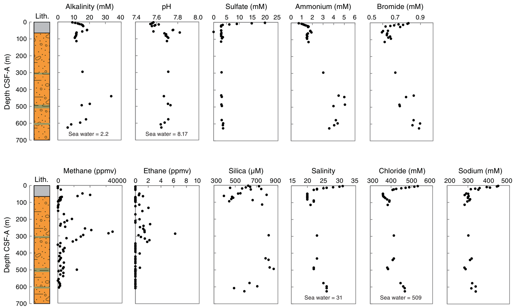
Figure F69. Dissolved chemical concentrations and headspace gas, Hole U1421A.
