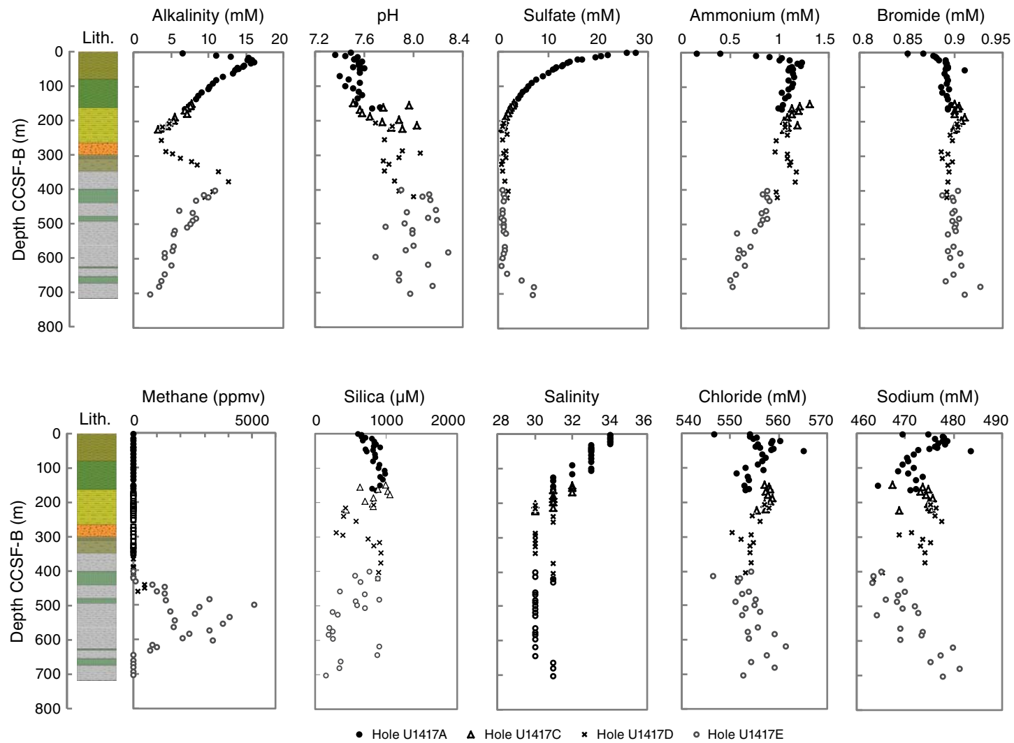
Figure F35. Dissolved chemical concentrations and headspace gas, Site U1417.
