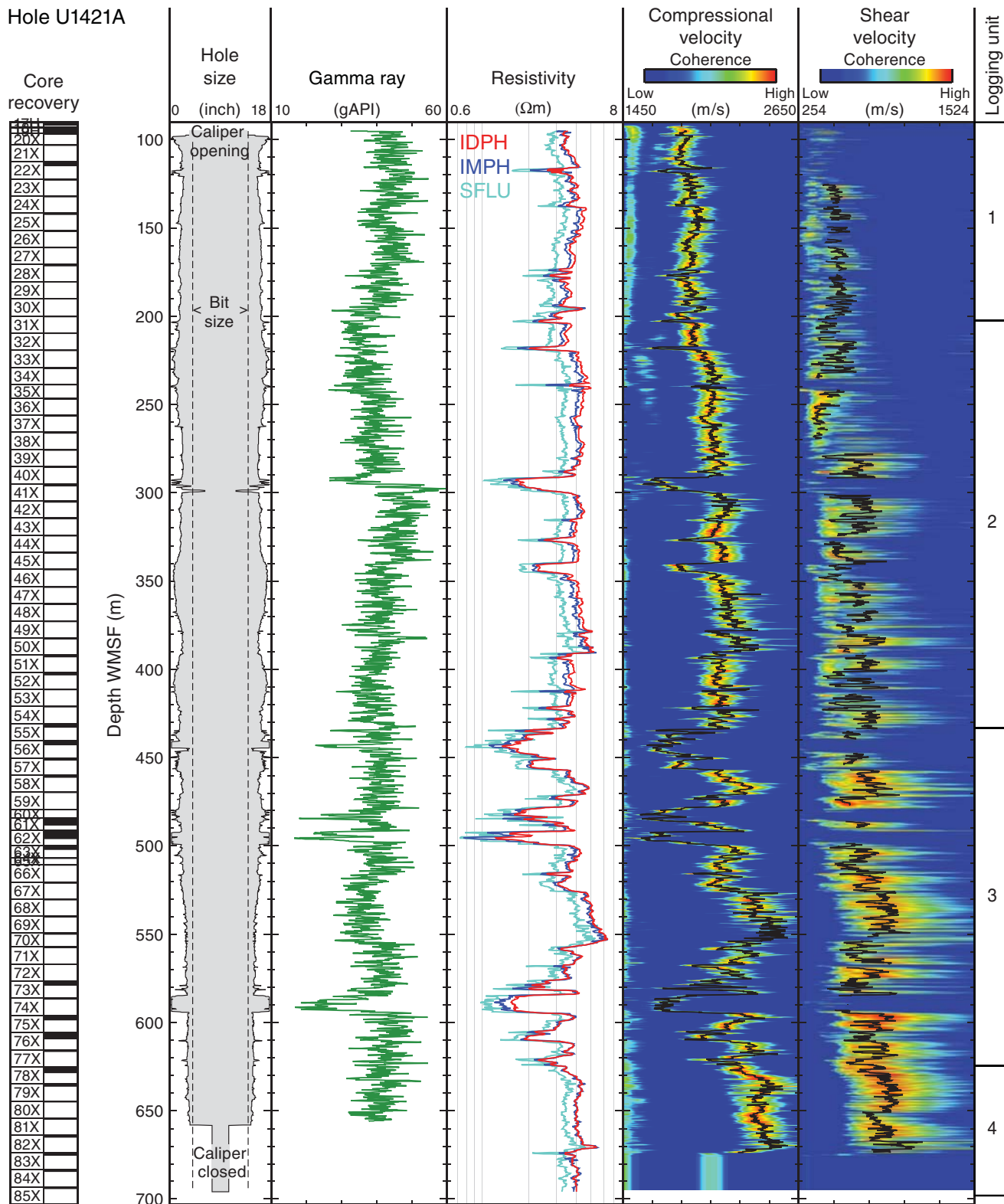
Figure F70. Summary of logs recorded by the sonic-induction tool string, Hole U1421A. Includes logs from the phasor dual induction–spherically focused resistivity tool: deep induction log (IDPH), medium induction log (IMPH), and shallow spherically focused resistivity log (SFLU). Logging units are also shown.
