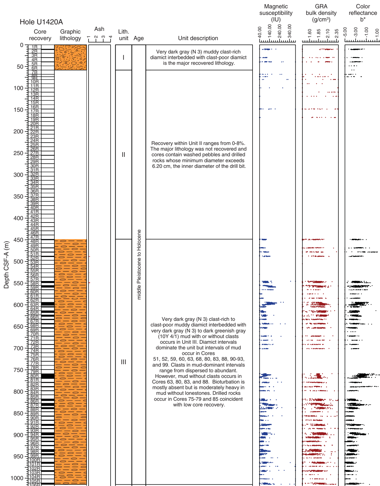
Figure F59. Core recovery, lithology, ash, lithologic units, age, unit descriptions, and physical properties data, Hole U1420A. ASH: 1 = trace, 2 = volcanoclastic bearing, 3 = volcanoclastic rich, 4 = ash. GRA = gamma ray attenuation.
