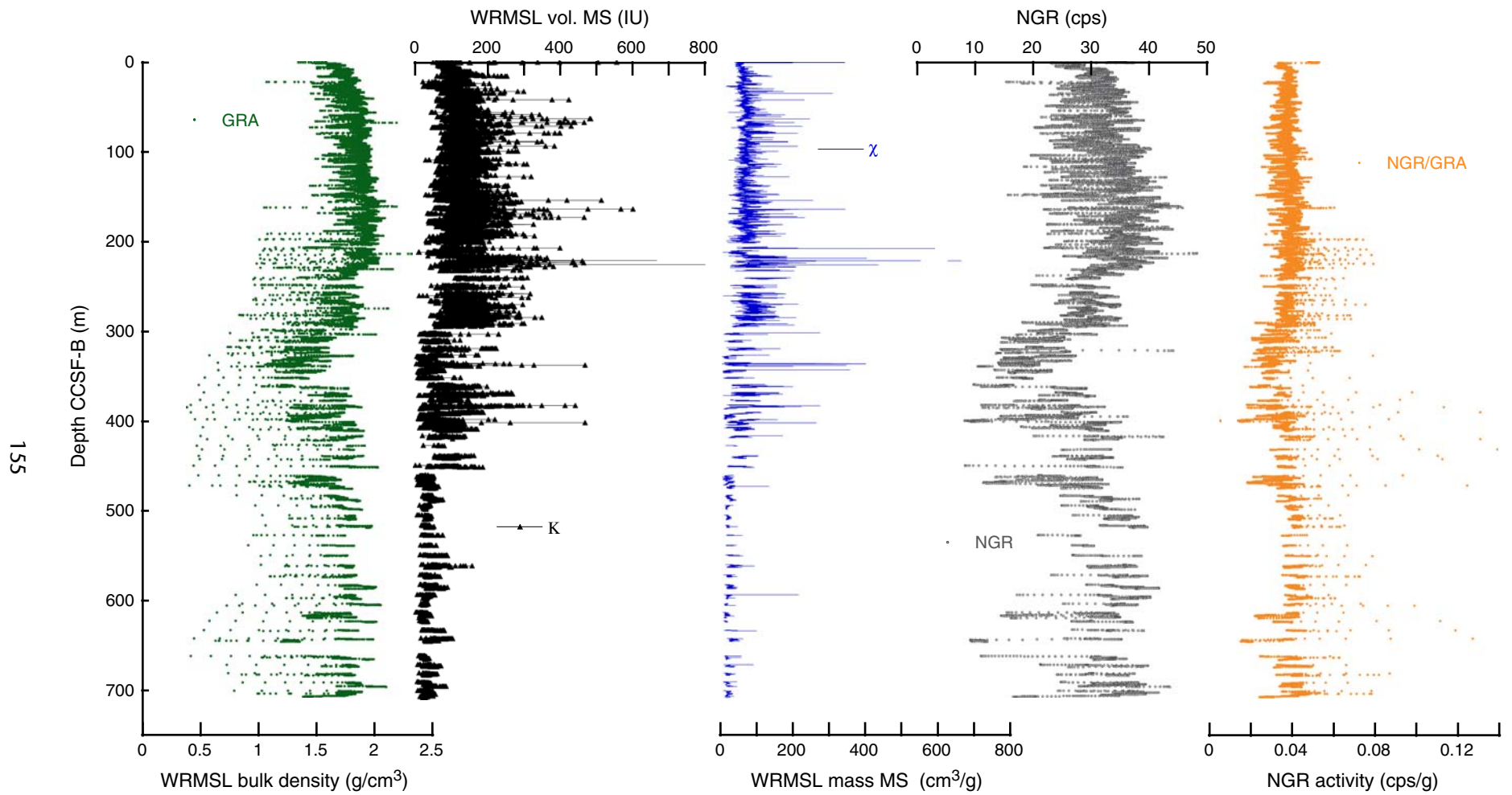
Figure F33. Whole-round Multisensor Logger (WRMSL) gamma ray attenuation (GRA) bulk density compared to WRMSL volume magnetic susceptibility (MS) data and natural gamma ray (NGR) data, Site U1417. Also shown are apparent GRA density-normalized WRMSL mass MS and NGR activity, corrected for variability in recovered sediment volume.
