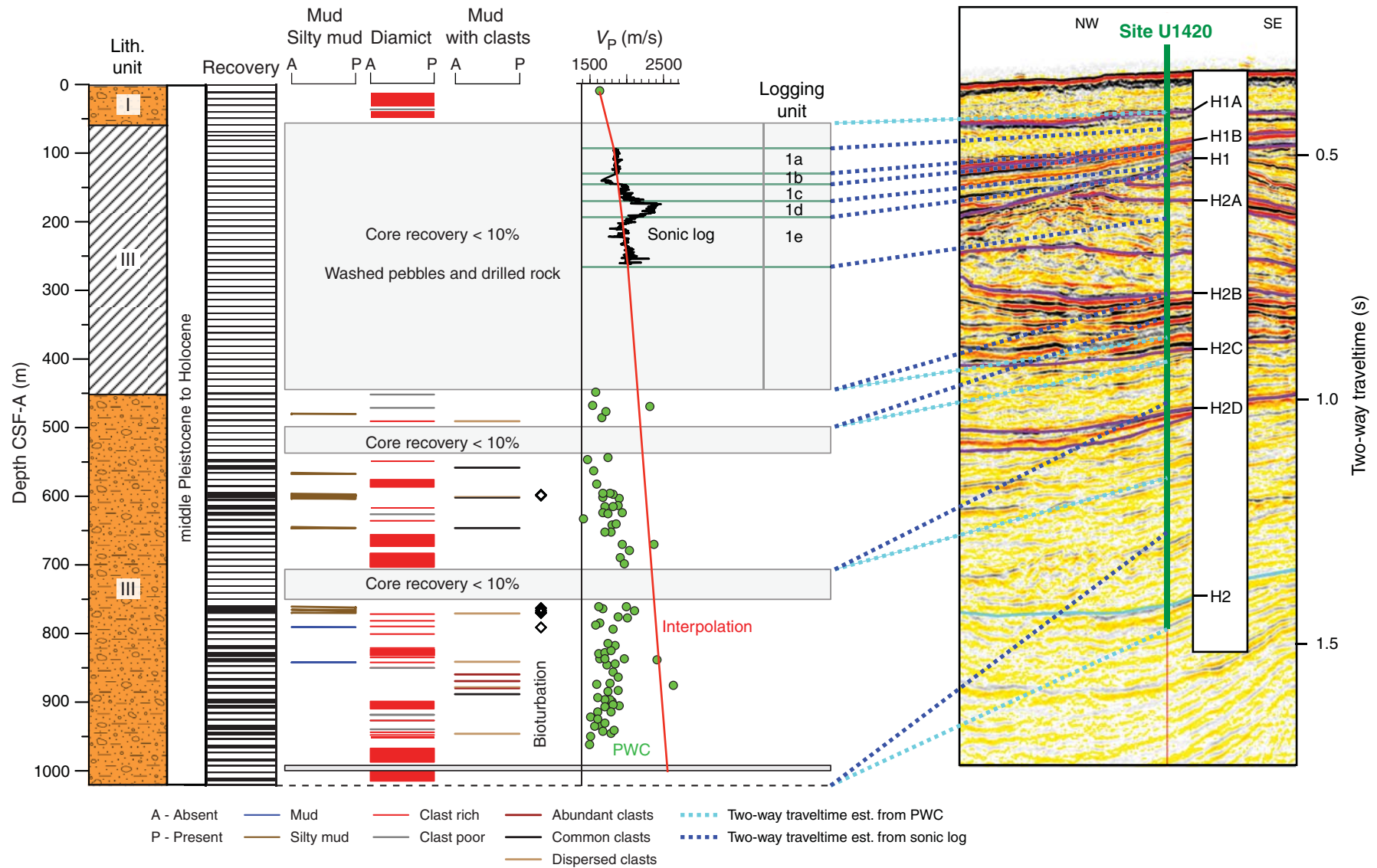
Figure F61. Integration of core, downhole logging, and seismic data, Site U1420. Two-way traveltime is calculated from P -wave caliper measurements (PWC) and sonic log velocities. Velocities were interpolated using downhole sonic log values where no data were available.
