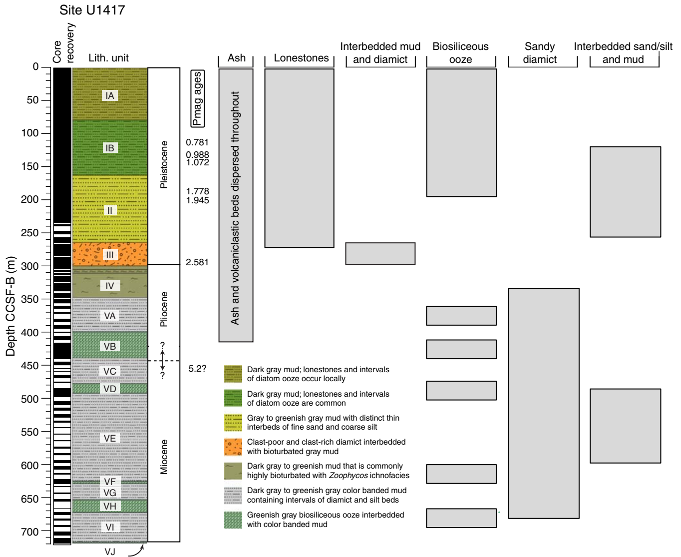
Figure F28. Site U1417 lithostratigraphic units and major lithologies used to define the lithostratigraphy, including ash and sediment containing volcanoclastic components, lonestones (>2 mm), diamict (ice-rafted interpretation), biosiliceous ooze, diamict (gravity flow interpretation), interbedded sand or silt with mud, and sand or silt beds. Data from all five holes were combined to produce a stratigraphic column showing the mid-depth location of each lithostratigraphic unit in the overall sedimentary sequence. Solid lines show where Neogene epoch boundaries coincide, or are within 10 m of a measured paleomagnetic reversal; dashed line separates the uncertain location of epoch boundaries estimated from the shipboard age model. Paleomagnetic age reversals in Ma are displayed to the right of the chronostratigraphic column.
