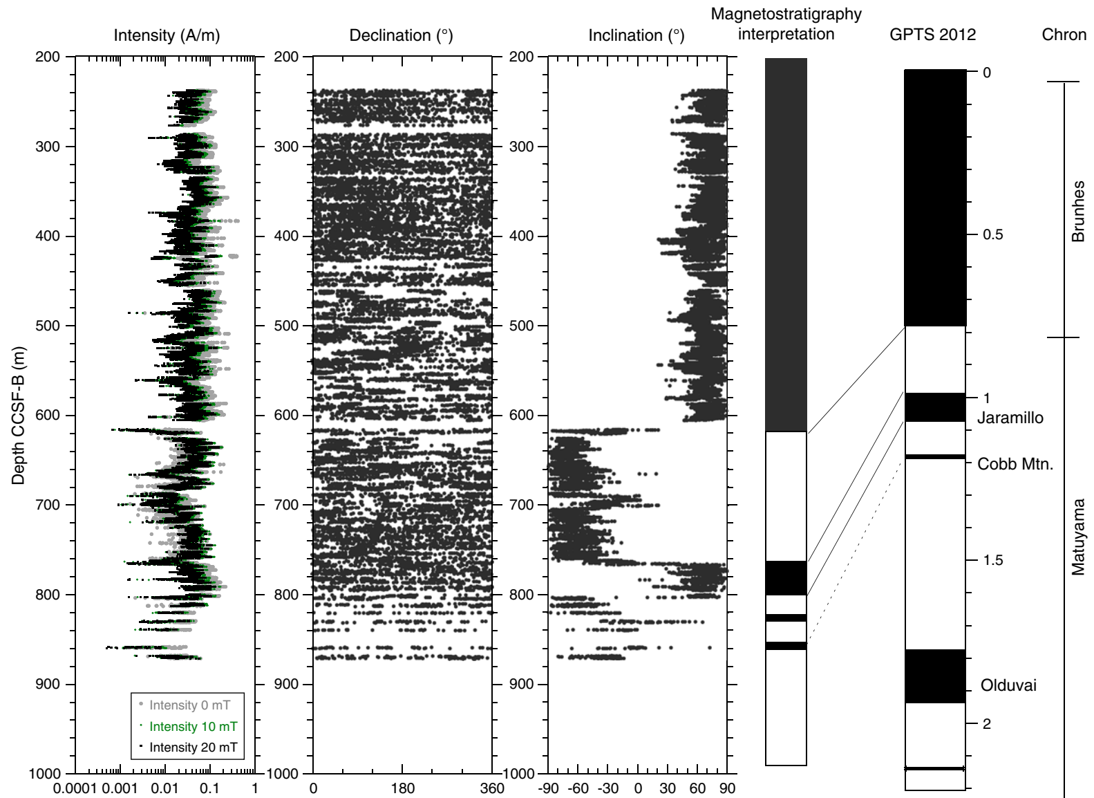
Figure F44. Intensity measured before and after 10 and 20 mT demagnetization, Hole U1418F. Declination and inclination measured after 20 mT peak AF demagnetization are also shown. GPTS 2012 from Hilgen et al. (2012). The bottom three Cores 341-U1418F-70R through 72R of mass transport deposit as chaotic unit are not included, though their intensities are similar.
