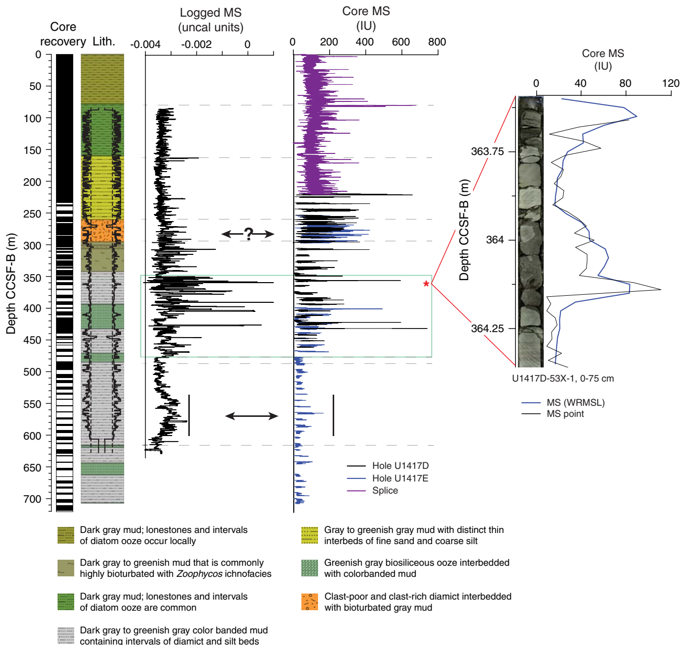
Figure F37. Lithostratigraphic units, borehole size, and core recovery, Site U1417. Magnetic susceptibility (MS) data were measured during downhole logging in Hole U1417E and on cores. Green rectangle = interval of clast-rich and clast-poor diamict interbedded with mud where magnetic susceptibility is highest and most variable in the logged data. Horizontal dashed lines = transitions between lithostratigraphic units. The inset figure highlights the correlation between diamict intervals and high magnetic susceptibility values in the core data. The core image is of Section 341-U1417D-53X-1, 0–75 cm, and the red star denotes its position. The inset figure provides evidence for the diamict intervals causing high magnetic susceptibility values in the logged data. A difference of as much as ~10 m may exist when comparing the CCSF-B and WMSL depth scales. WRMSL = Whole-Round Multisensor Logger.
