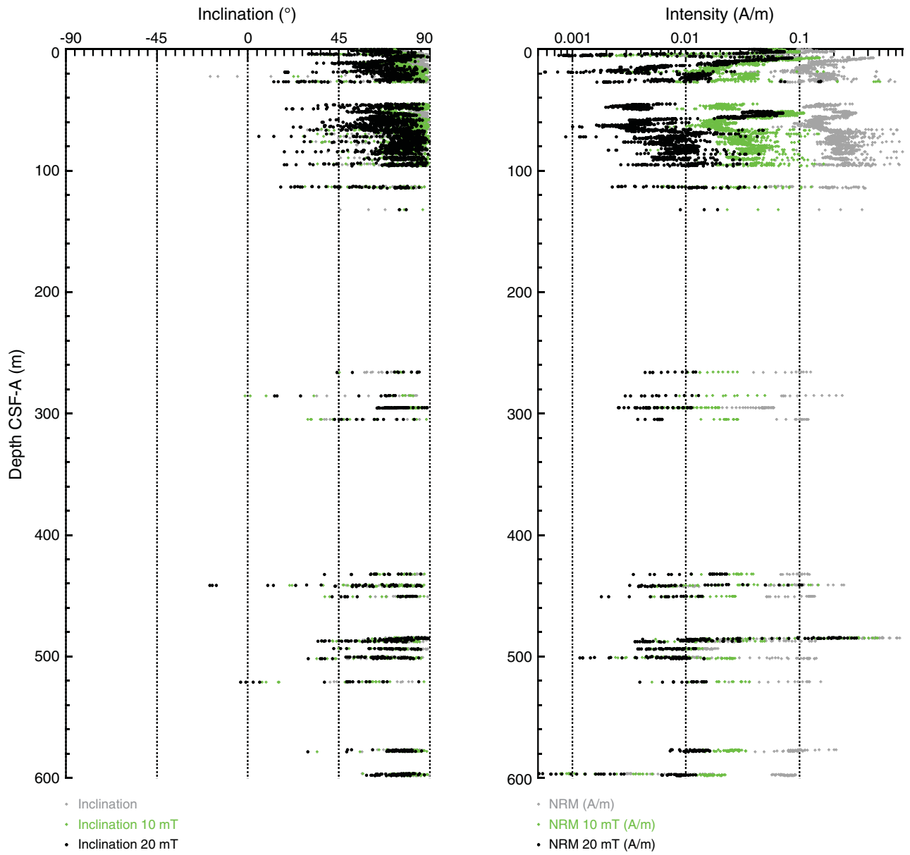
Figure F68. Natural remanent magnetization (NRM) intensities and inclination measured before and after 10 and 20 mT peak AF demagnetization, Hole U1421A.
