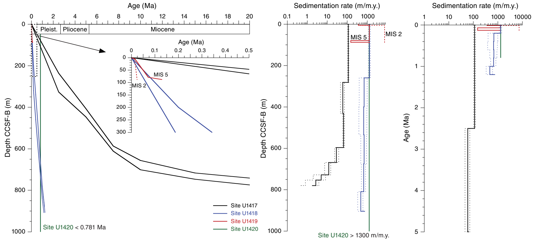
Figure F21. Expedition 341 age-depth plots and sedimentation summary. Minimum and maximum rates are shown for each site. MIS = marine isotope stage.
