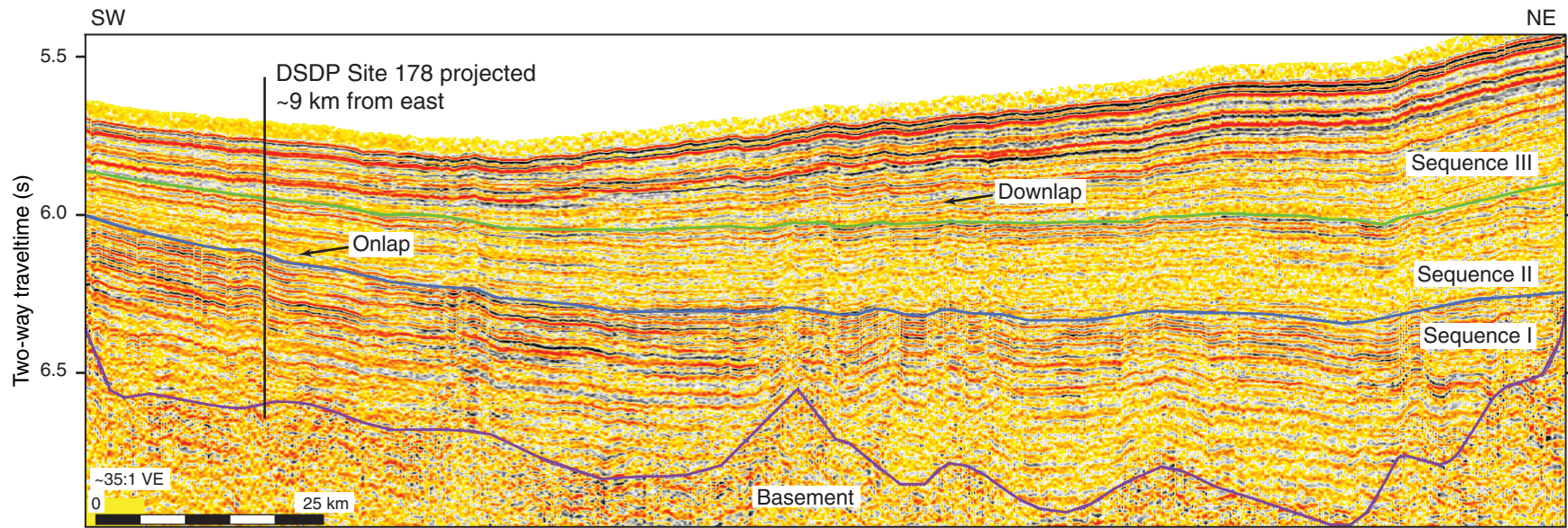
Figure F15. Seismic reflection Line 13 from 1989 USGS Survey F689 showing sequences newly defined by Reece et al. (2013) and approximate correlation to DSDP Site 178. See Figure F6 for line location. Vertical exaggeration (VE) assumes 2000 m/s sediment acoustic velocity. Modified from Reece et al. (2011).
