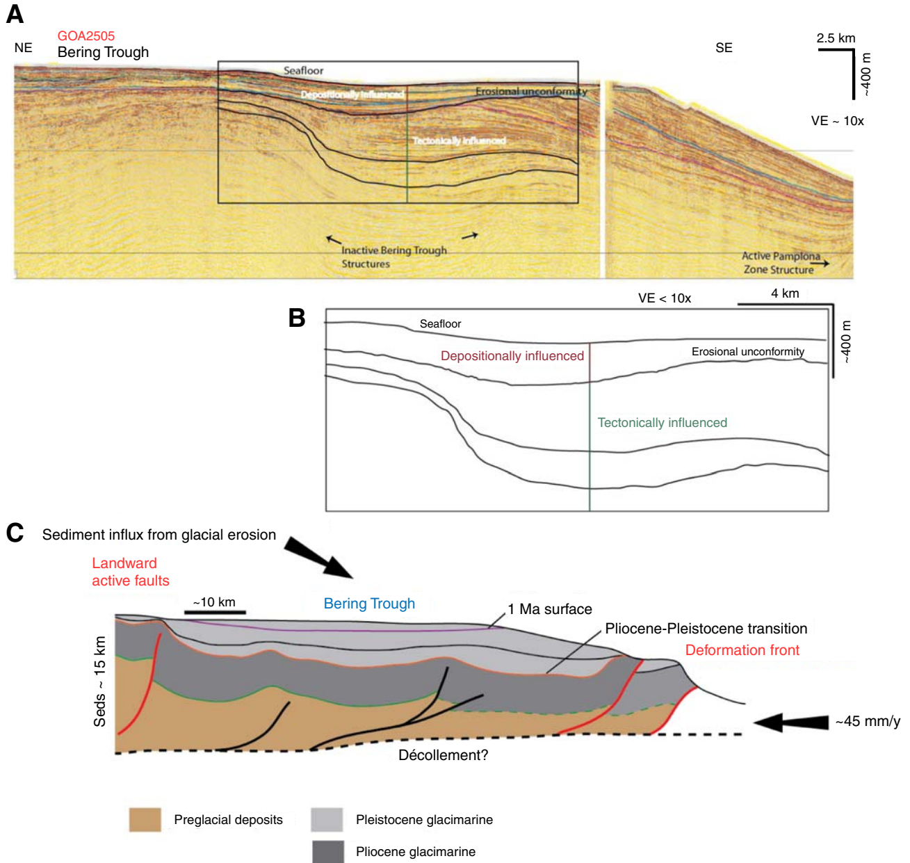
Figure F12. Seismic Profile GOA-2505. VE = vertical exaggeration. A. High-resolution seismic imaging Bering Trough showing a distinct change in margin architecture from tectonically to depositionally influenced at the labeled erosional unconformity. B. Interpretations for seismic Profile GOA-2505. Location of seismic profile shown in Figure F1. C. Schematic cross-section across frontal St. Elias wedge. Sed. = Neogene sediments. Modified from Worthington et al., 2008, 2010.
