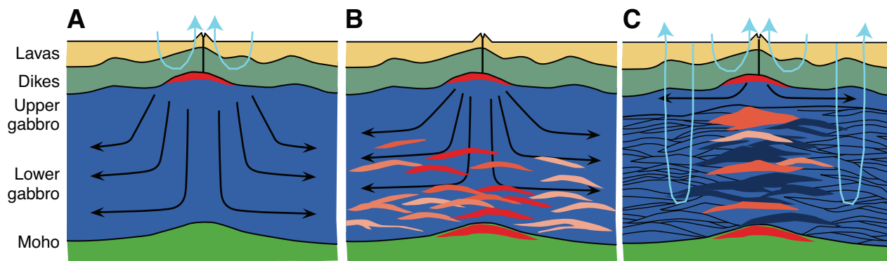
Figure F2. Schematic drawings of crustal accretion models (modified from Korenaga and Kelemen, 1997). Black arrows = movement of the crystal mush, blue arrows = dominant zones where hydrothermal circulation removes latent and sensible heat. A. Gabbro glacier in which the lower oceanic crust crystallizes in a thin magma lens at the base of the sheeted dike complex from which cumulates subside downward and outward to form the lower crust (e.g., Henstock et al., 1993; Phipps Morgan and Chen, 1993; Quick and Denlinger, 1993). B. Hybrid model in which some crystallization occurs in an upper melt lens and some within sill-like bodies in the lower crust (e.g., Boudier et al., 1996). C. “Sheeted” or “stacked” sill model in which the lower ocean crust forms by crystallization of multiple sill-like intrusions (e.g., Bédard et al., 1988; Kelemen and Aharonov, 1998; Kelemen et al., 1997).
