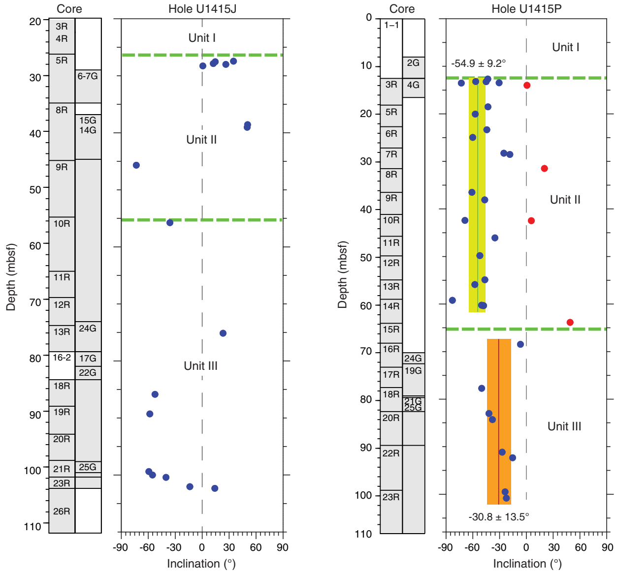
Figure F23. Plots of variation with depth of the inclination of high unblocking temperature components of magnetization in discrete samples, Holes U1415J and U1415P. Data from Hole U1415J show a downhole change from an upper unit with downward-directed magnetization to a lower unit with upward-directed magnetization, suggesting sampling of blocks that have been inverted relative to each other. More extensive data from Hole U1415P allow definition of statistically different mean inclinations from petrologically defined Units I (Layered Series) and III (Troctolitic Series), again consistent with sampling of two blocks with independent rotation histories.
