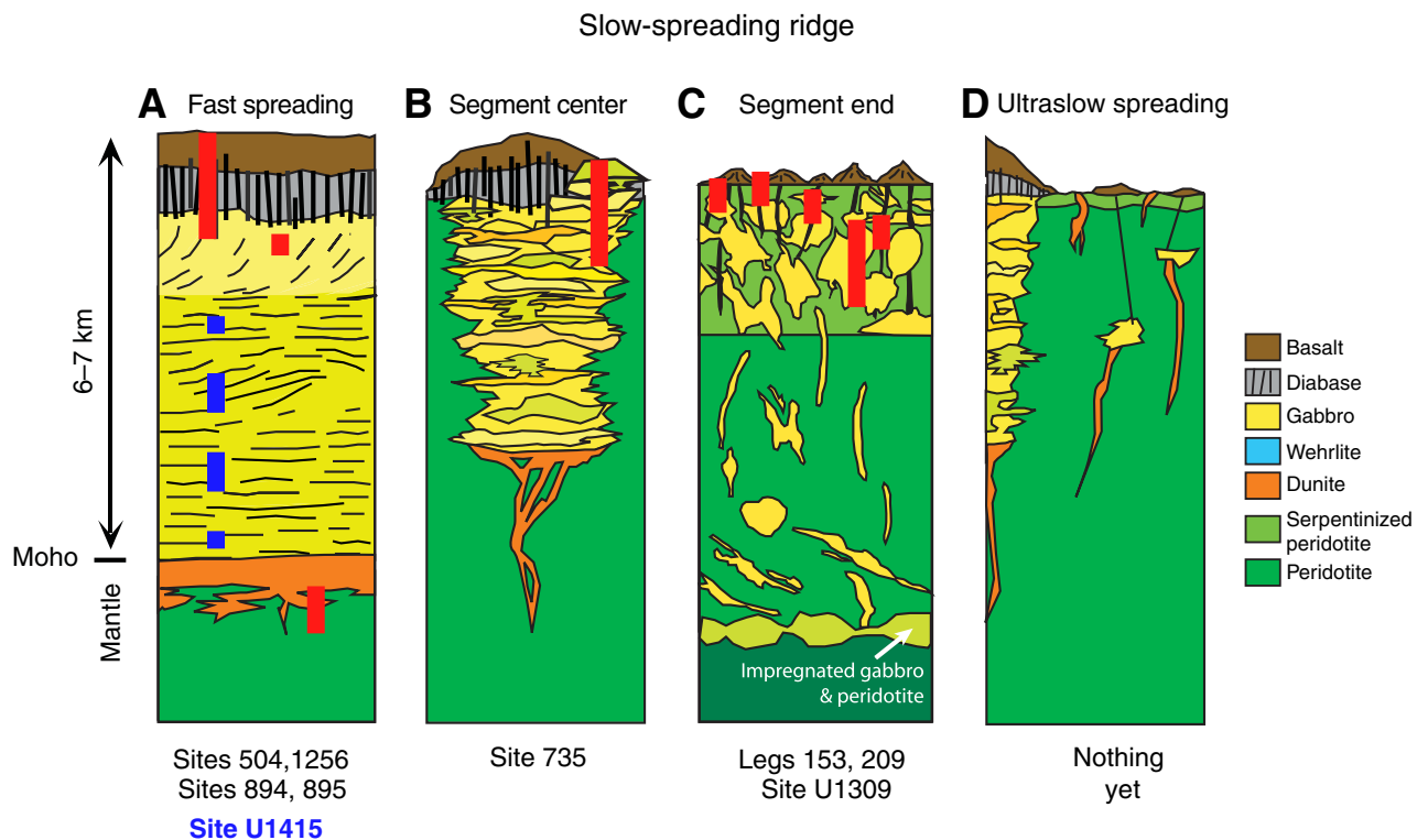
Figure F1. Schematic models for the ocean crust showing how its structure changes with decreasing magmatism and increasing faulting from A to D. Modified after Dick et al. (2007). A. Fast-spreading crust, after the Penrose standard layered model (Anonymous, 1972). Red bars = major deep drilling sites, dashed blue bar = drilling target area for Expedition 345. Moho = Mohorovicic discontinuity. B. Slow-spreading crust formed at a segment center (Cannat et al., 1995). C. Slow-spreading crust formed at a segment end (Cannat et al., 1995). D. Ultraslow-spreading crust, which is the nearly nonvolcanic end-member of crustal construction (Dick et al., 2007).
