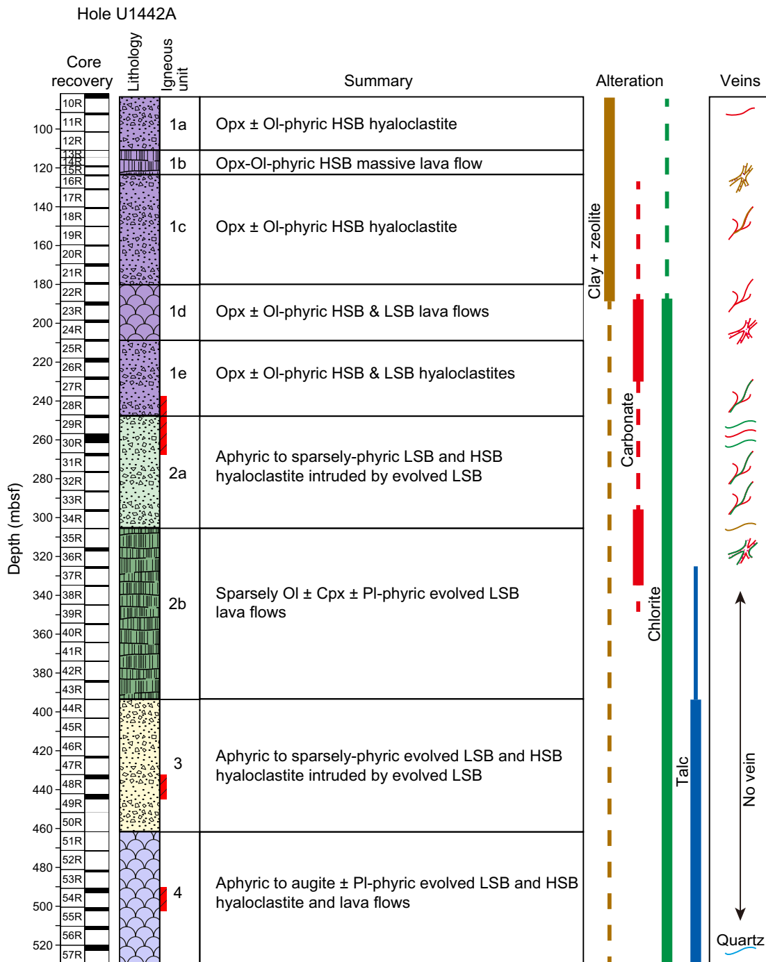
Figure F18. Lithostratigraphic igneous units, Hole U1442A. Red bars adjacent to lithology column represent fault zones.
