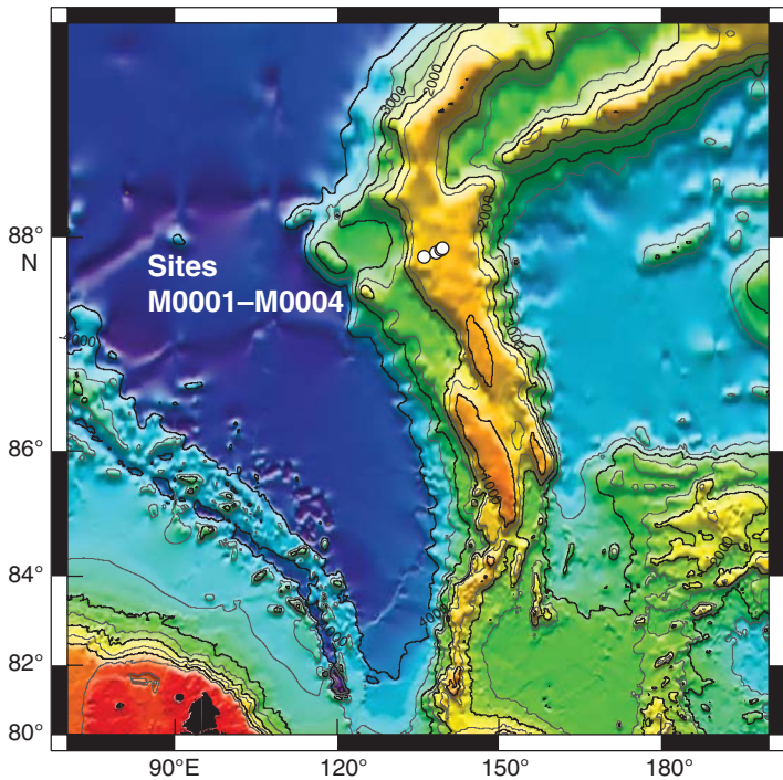
IODP Expedition 302 Site Map
