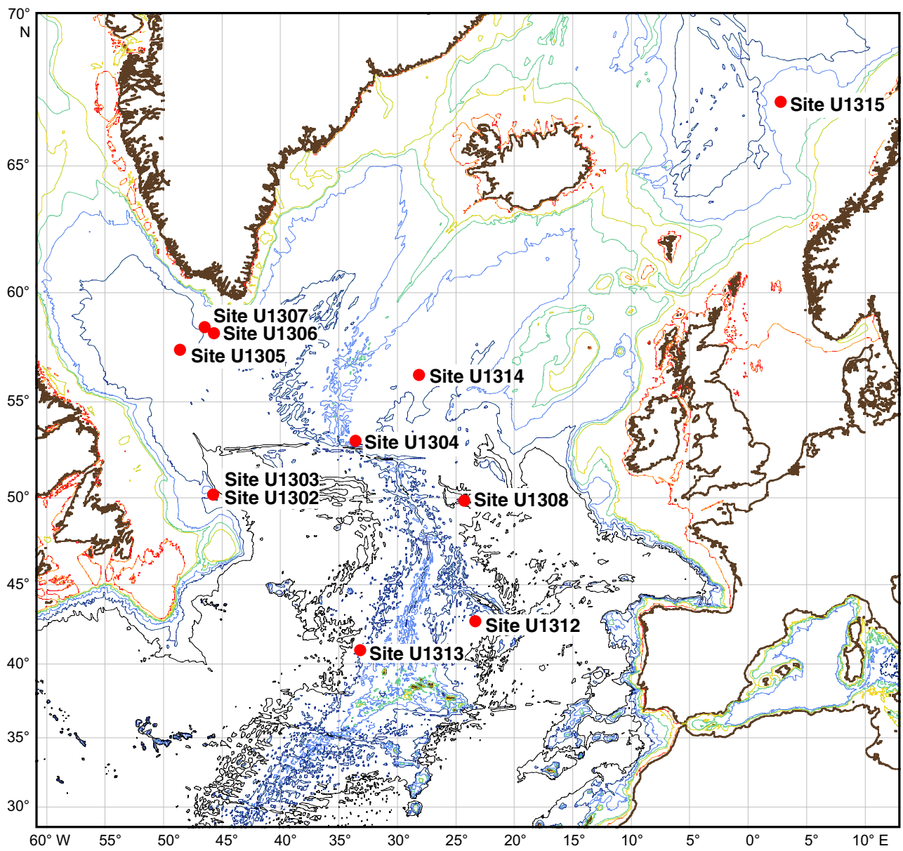
IODP Expedition 303/306 Site Map
