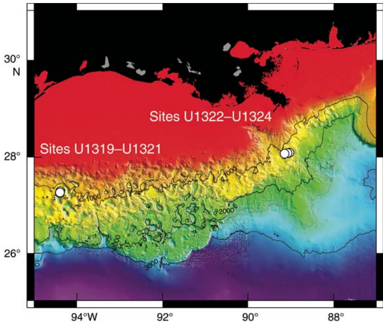
IODP Expedition 308 Site Map
