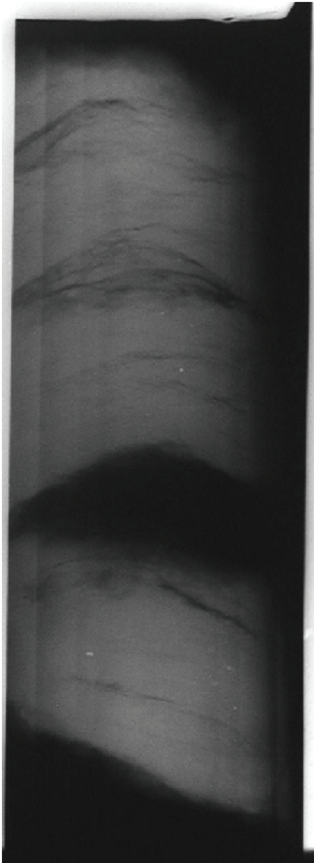
Radiograph U1319A_12H_CC, 4 to 21 cm, 106.27-106.44 mbsf
