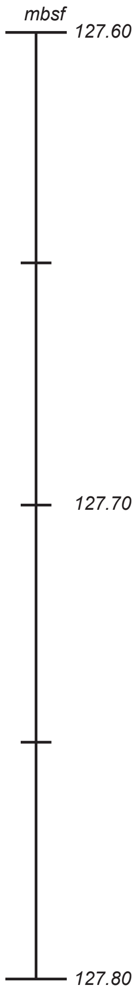
Radiograph U1320A_16X_1, 130 to 150 cm, 127.60-127.80 mbsf
