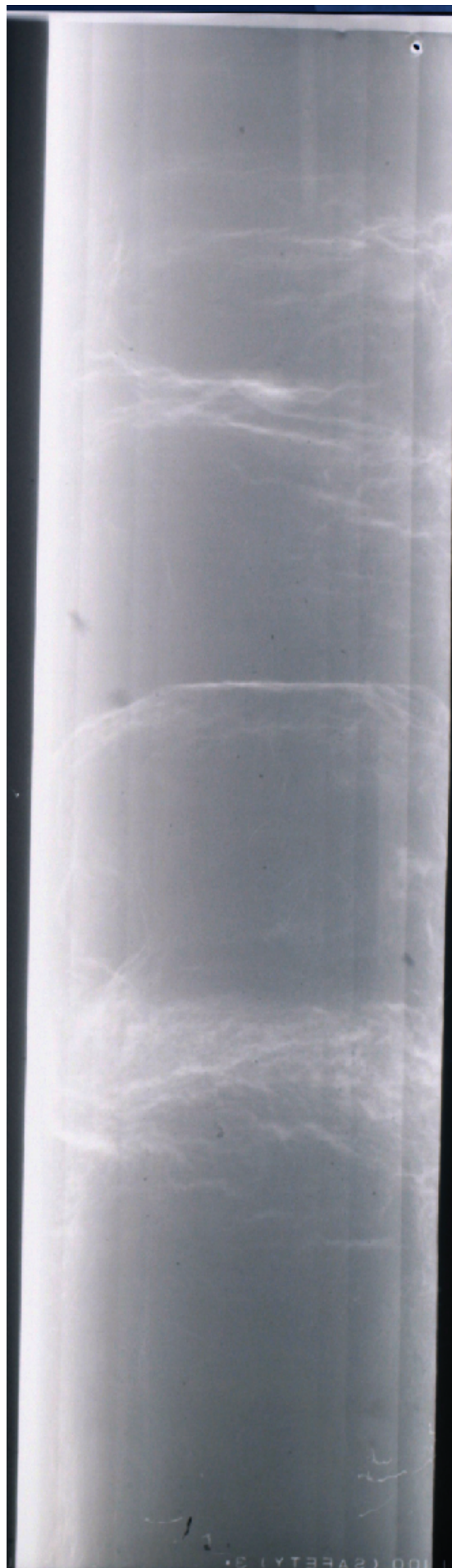
Radiograph U1320A_32X_6, 25 to 50 cm, 287.55-287.80 mbsf
