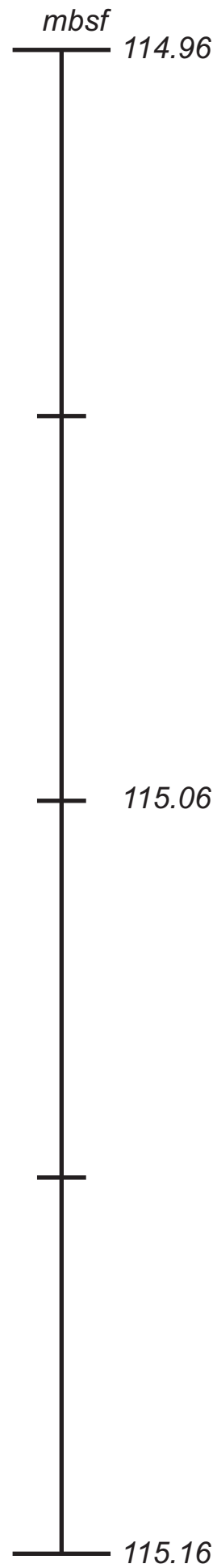
Radiograph U1322B_13H_6, 40 to 60 cm, 114.96-115.16 mbsf
