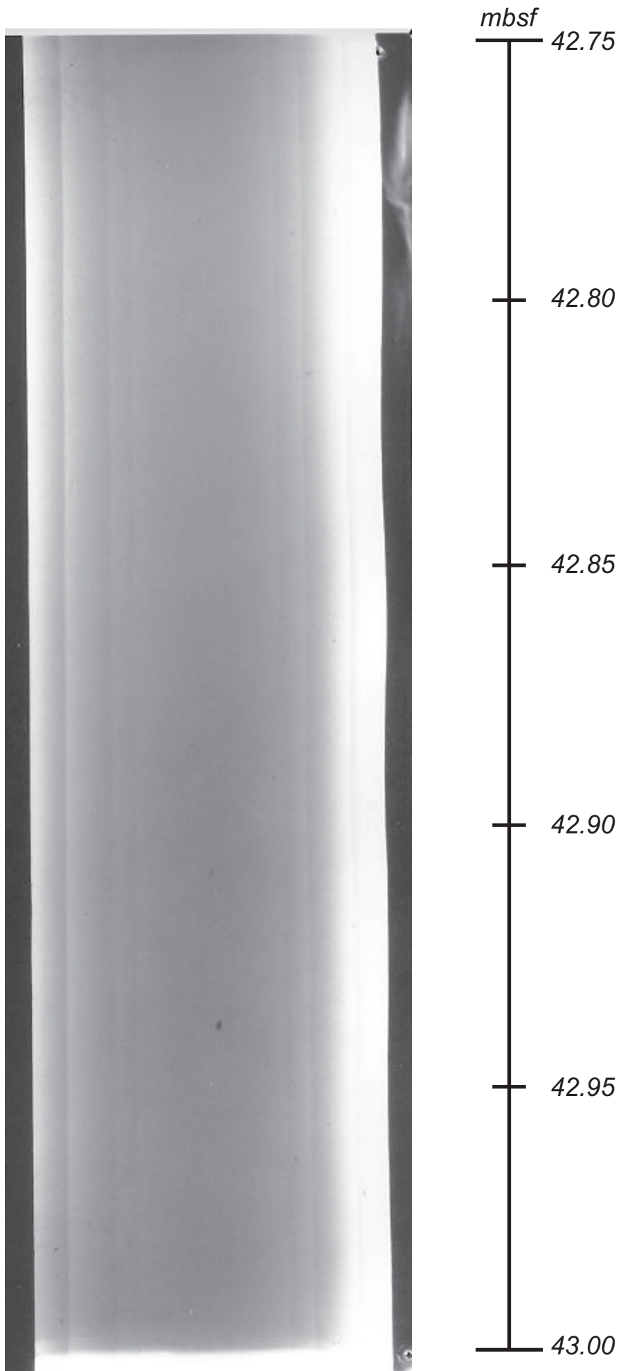
Radiograph U1322D_1H_2, 125 to 150 cm, 42.75-43.00 mbsf
