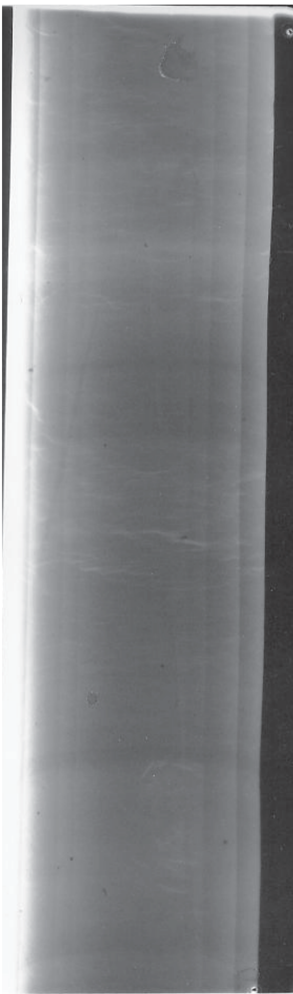
Radiograph U1322D_2H_2, 100 to 125cm, 72.50-72.75 mbsf
