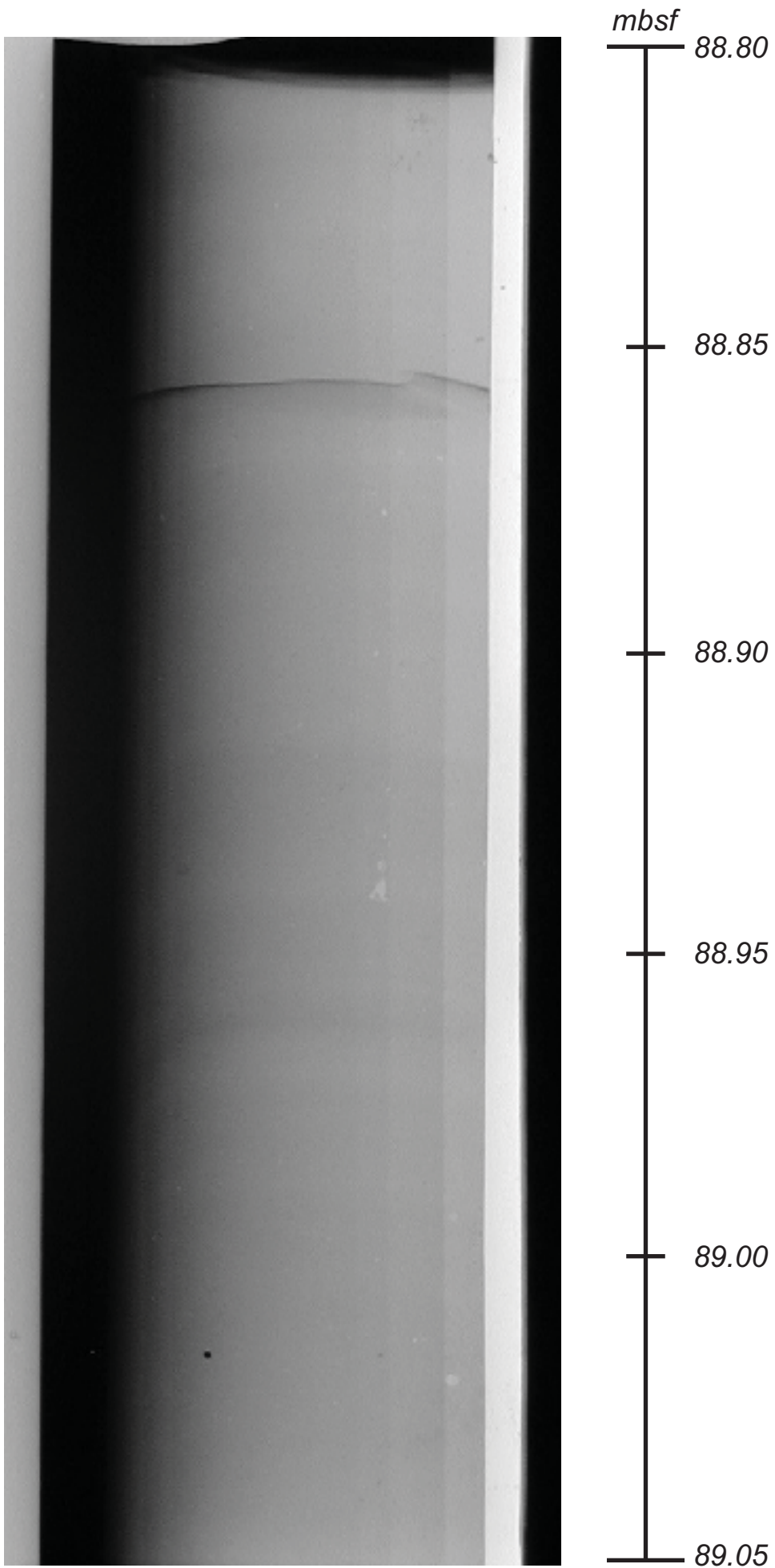
Radiograph U1324B_10H_7, 0 to 25 cm, 88.80-89.05 mbsf
