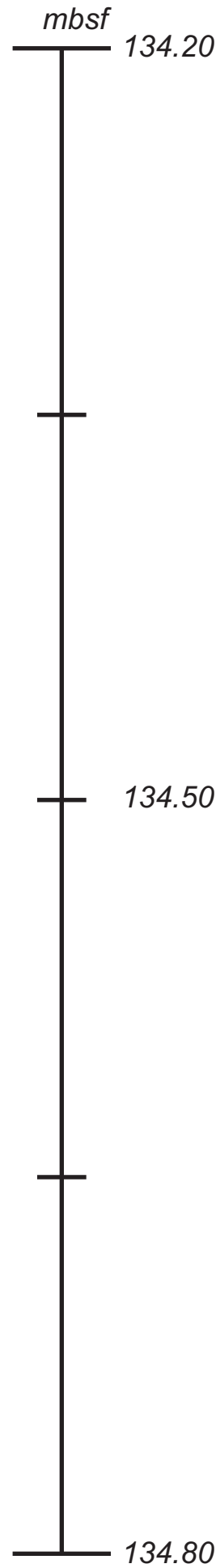
Radiograph U1324B_15H_5, 90 to 150 cm, 134.20-134.80 mbsf
