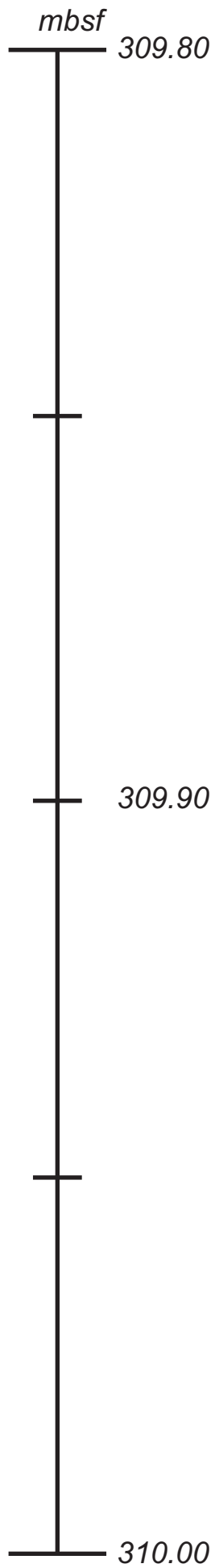
Radiograph U1324B_37H_3, 120 to 140 cm, 309.80-310.00 mbsf
