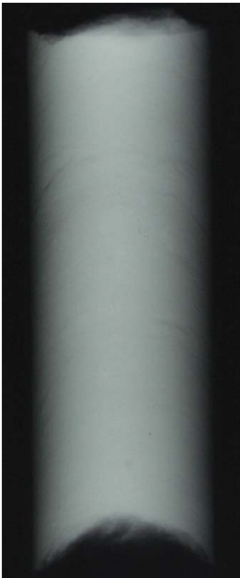
Radiograph U1324B_37H_3, 120 to 140 cm, 309.80-310.00 mbsf
