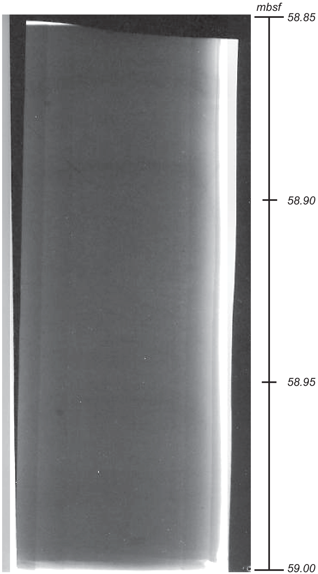
Radiograph U1324C_1H_6, 135 to 150 cm, 58.85-59.00 mbsf
