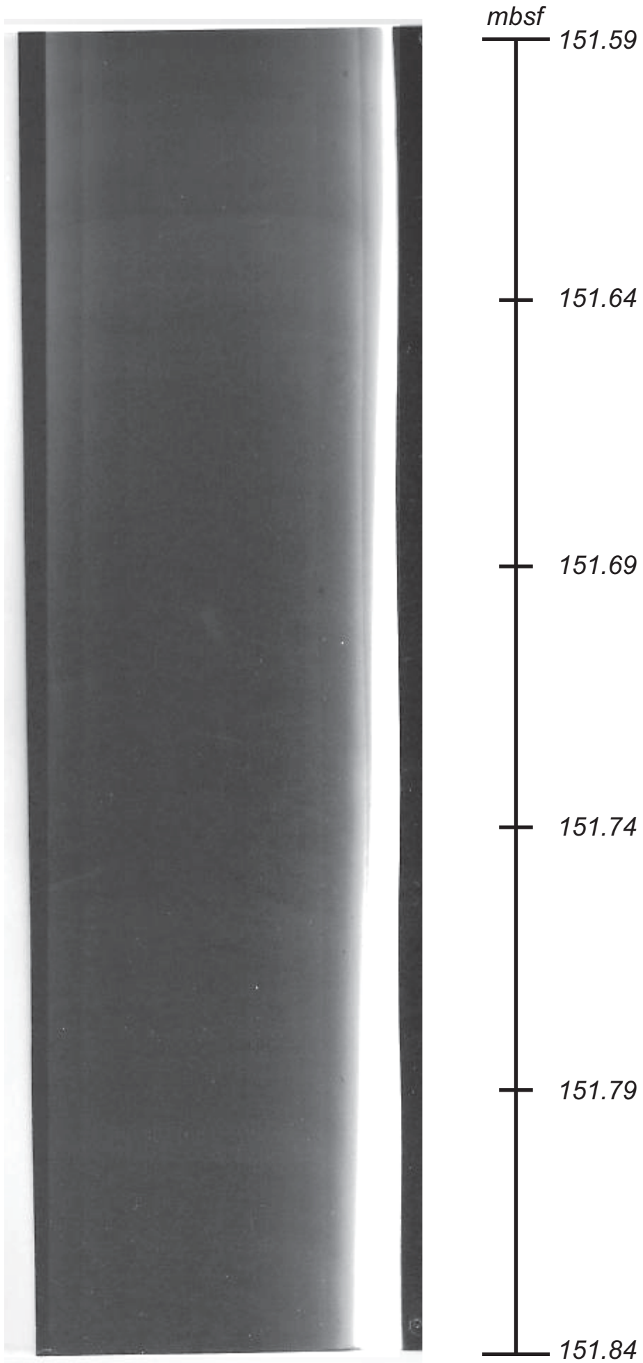
Radiograph U1324C_3H_2, 100 to 125 cm, 151.59-151.84 mbsf
