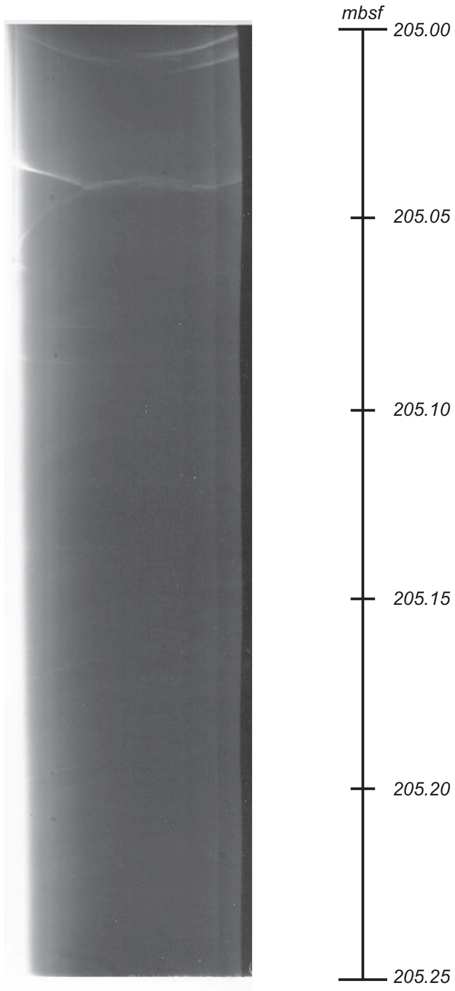
Radiograph U1324C_4H_4, 50 to 75 cm, 205.00-205.25 mbsf
