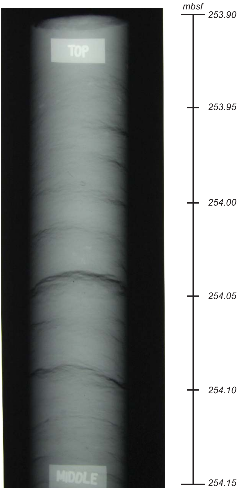
Radiograph U1324C_5H_3, 90 to 115 cm, 253.90-254.15 mbsf
