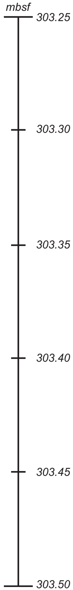
Radiograph U1324C_6H_3, 25 to 50 cm, 303.25-303.50 mbsf
