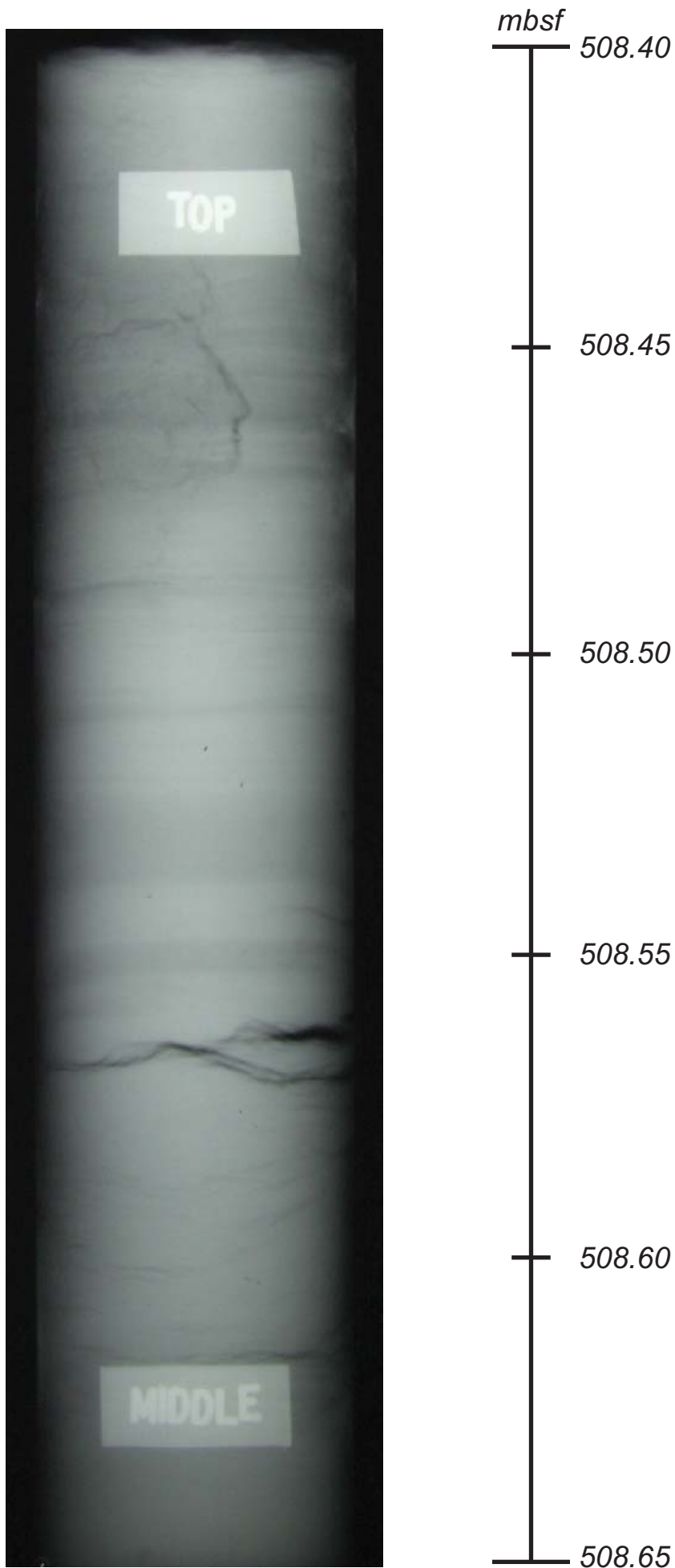
Radiograph U1324C_8H_3, 40 to 65 cm, 508.40-508.65 mbsf
