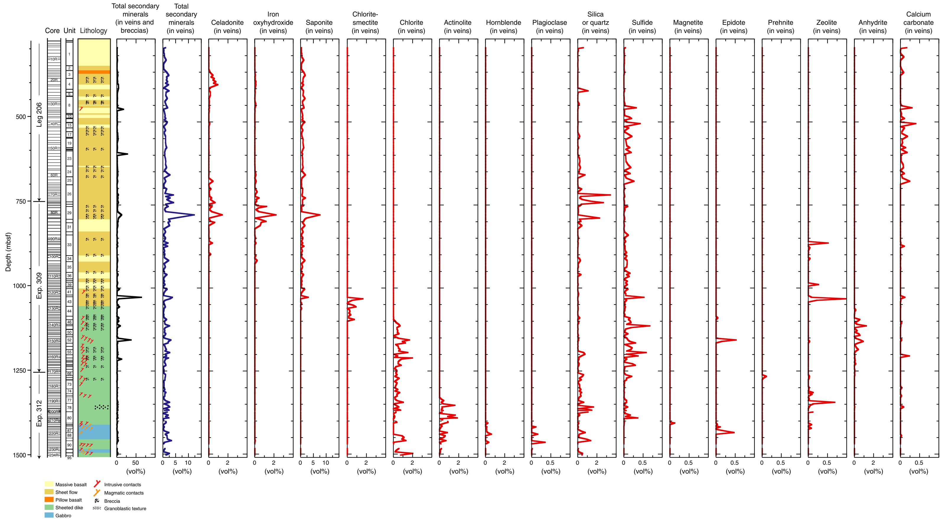
Expedition 309/312 summary, Figure F43. Total volume percent of secondary minerals contained within veins in Hole 1256D. Percentages are normalized to amount of recovered material per core (per meter) and plotted vs. depth to top of core.
