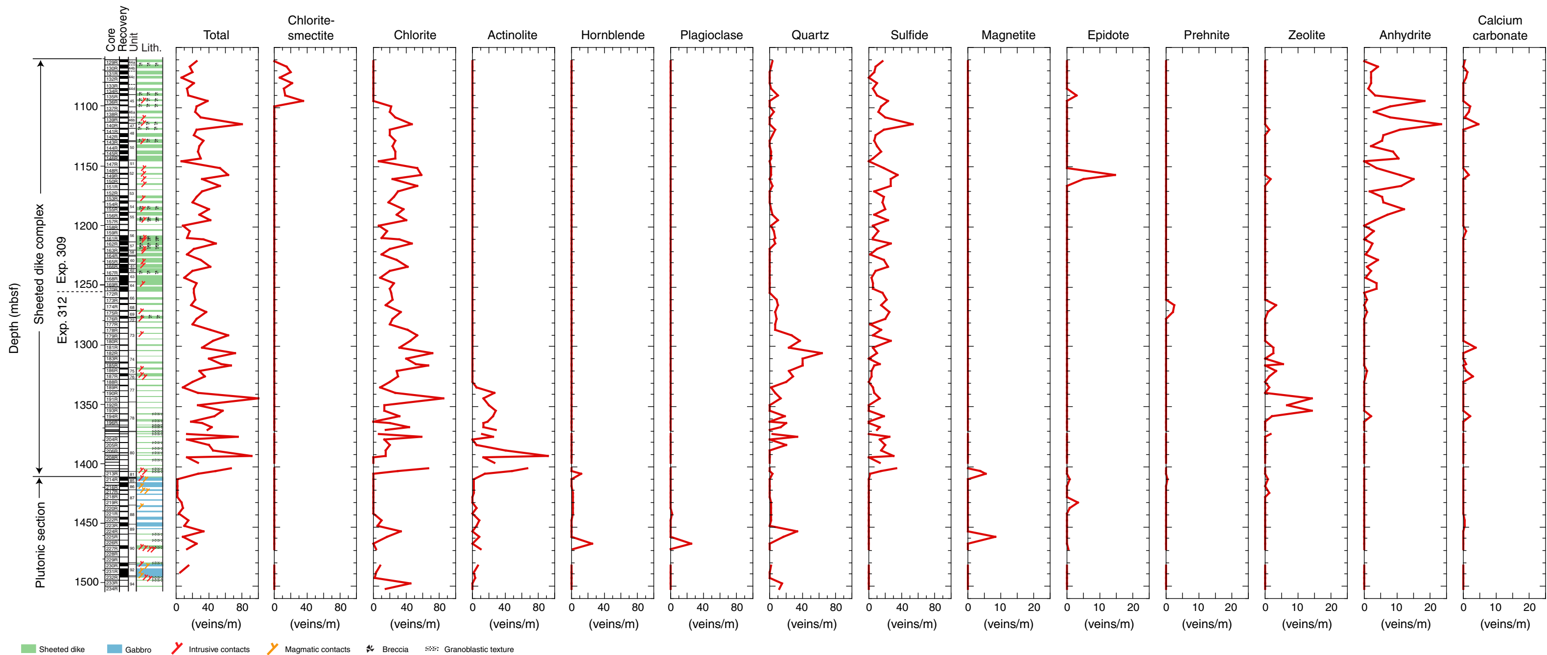
Site 1256, Figure F259. Abundance of secondary mineral veins with depth in the sheeted dike complex and plutonic section of Hole 1256D. Numbers of veins are normalized to amount of recovered material per core (veins per meter).
