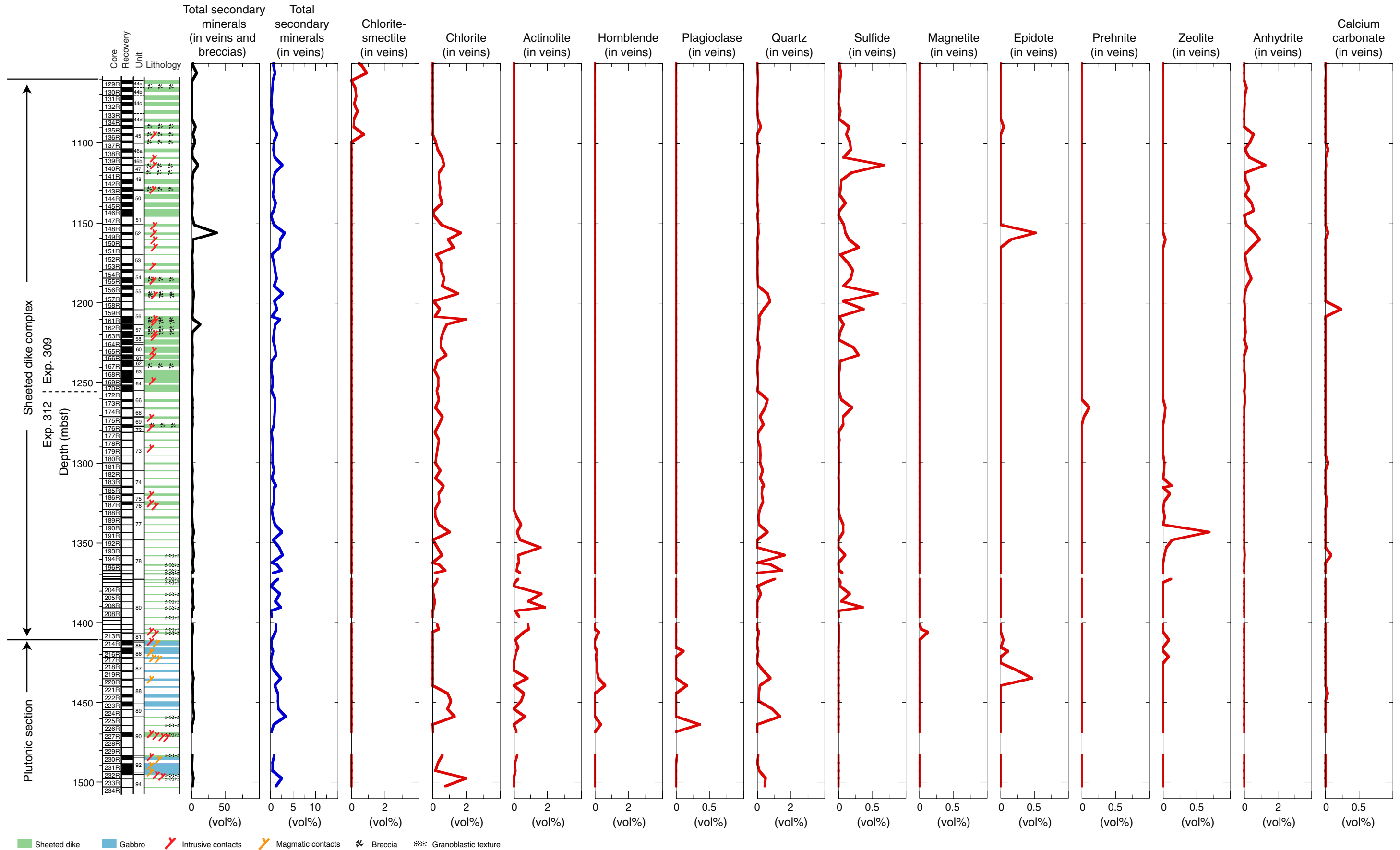
Site 1256, Figure F260. Total volume percent of secondary minerals contained within veins and veins plus breccias with depth in the sheeted dike complex and plutonic section of Hole 1256D (given as volume percentage of recovered core, per core).
