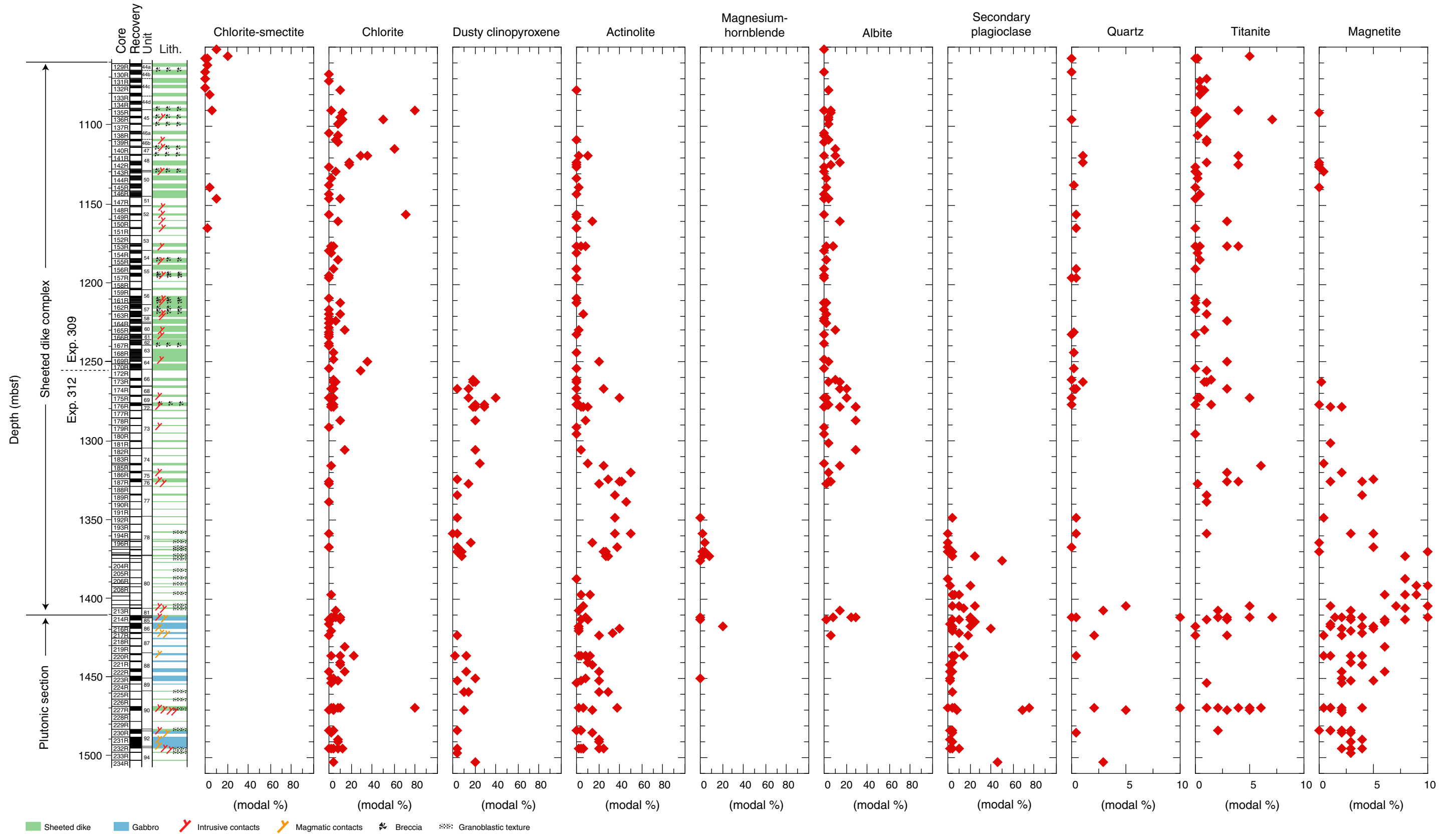
Site 1256, Figure F261. Modal mineral abundance with depth in the sheeted dike complex and plutonic section of Hole 1256D tabulated from thin section observations. Note that, although present, dusty clinopyroxene was not recorded in thin section descriptions from Expedition 309.
