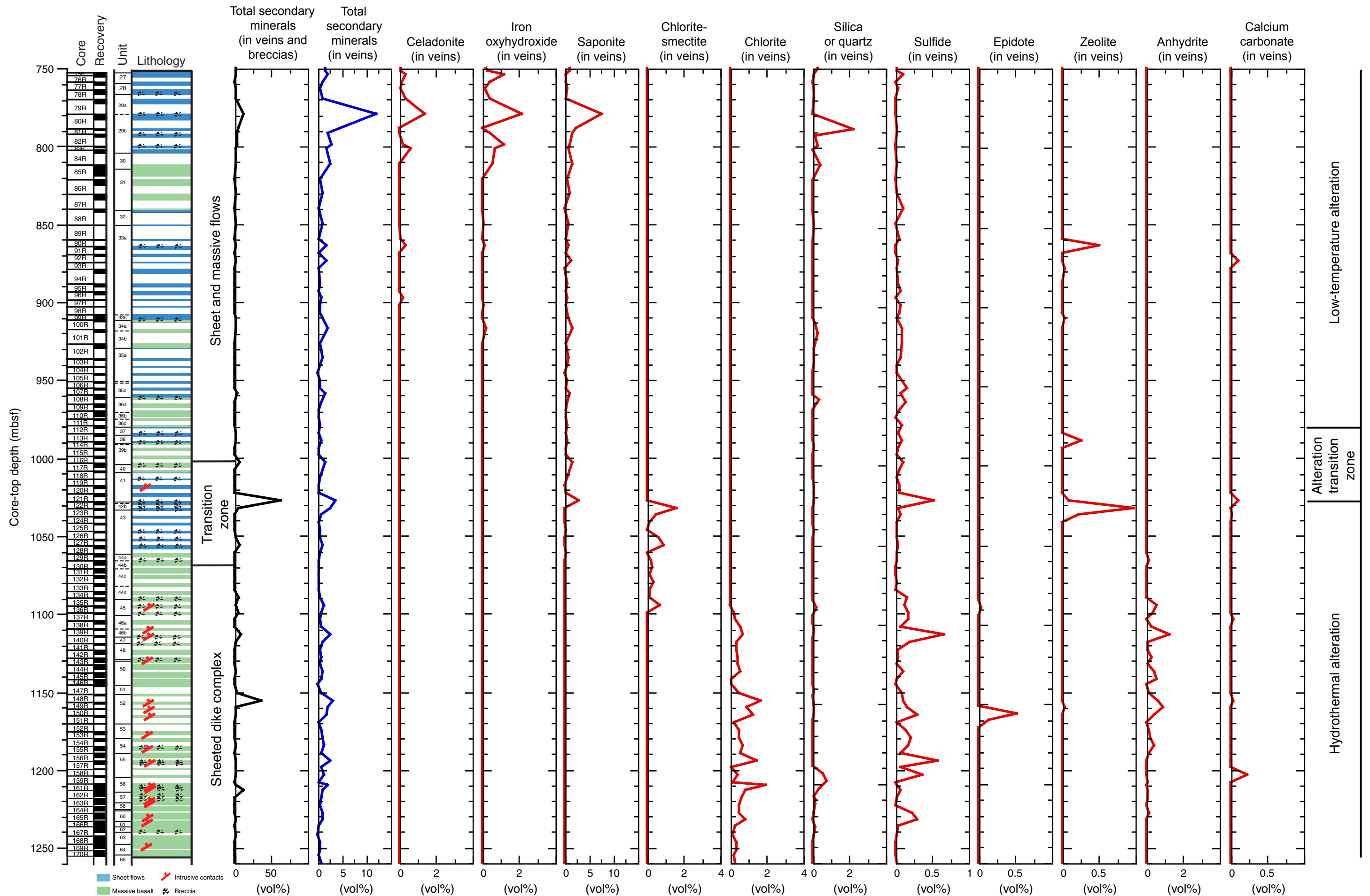
Site 1256, Figure F81. Total volume percent of secondary minerals composing veins with depth in Hole 1256D (Expedition 309). Percentages are normalized to amount of recovered material per core (per meter) and plotted vs. depth to the top of the core.
