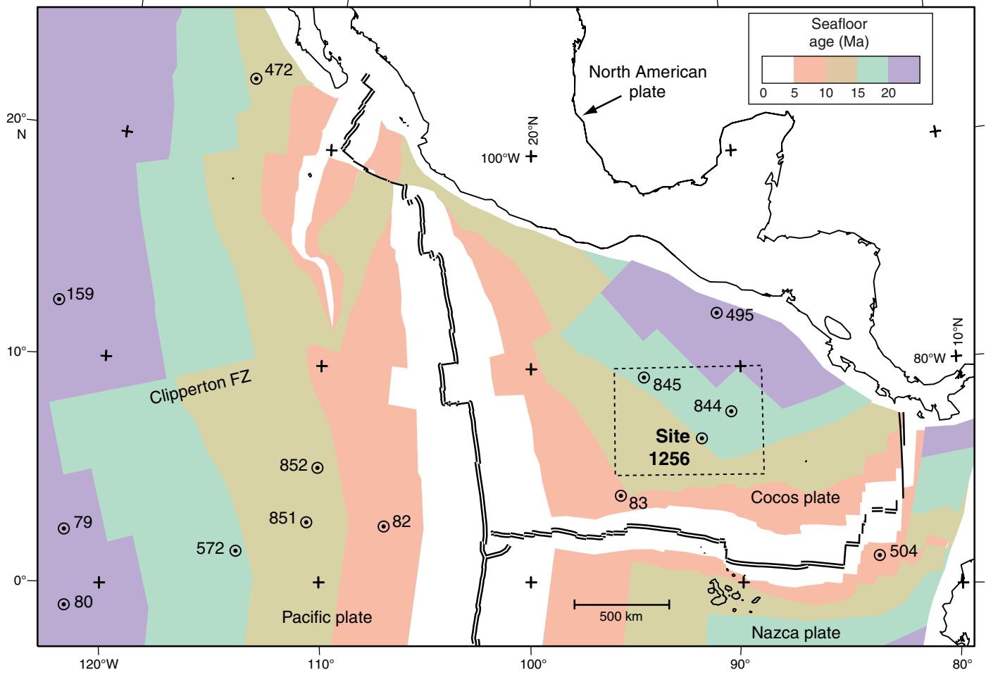
IODP Expedition 309/312 Site Map
