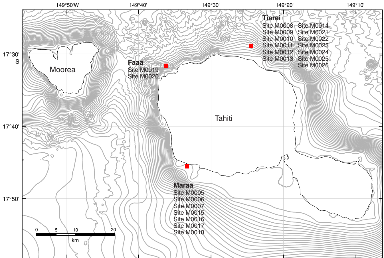
IODP Expedition 310 Site Map
