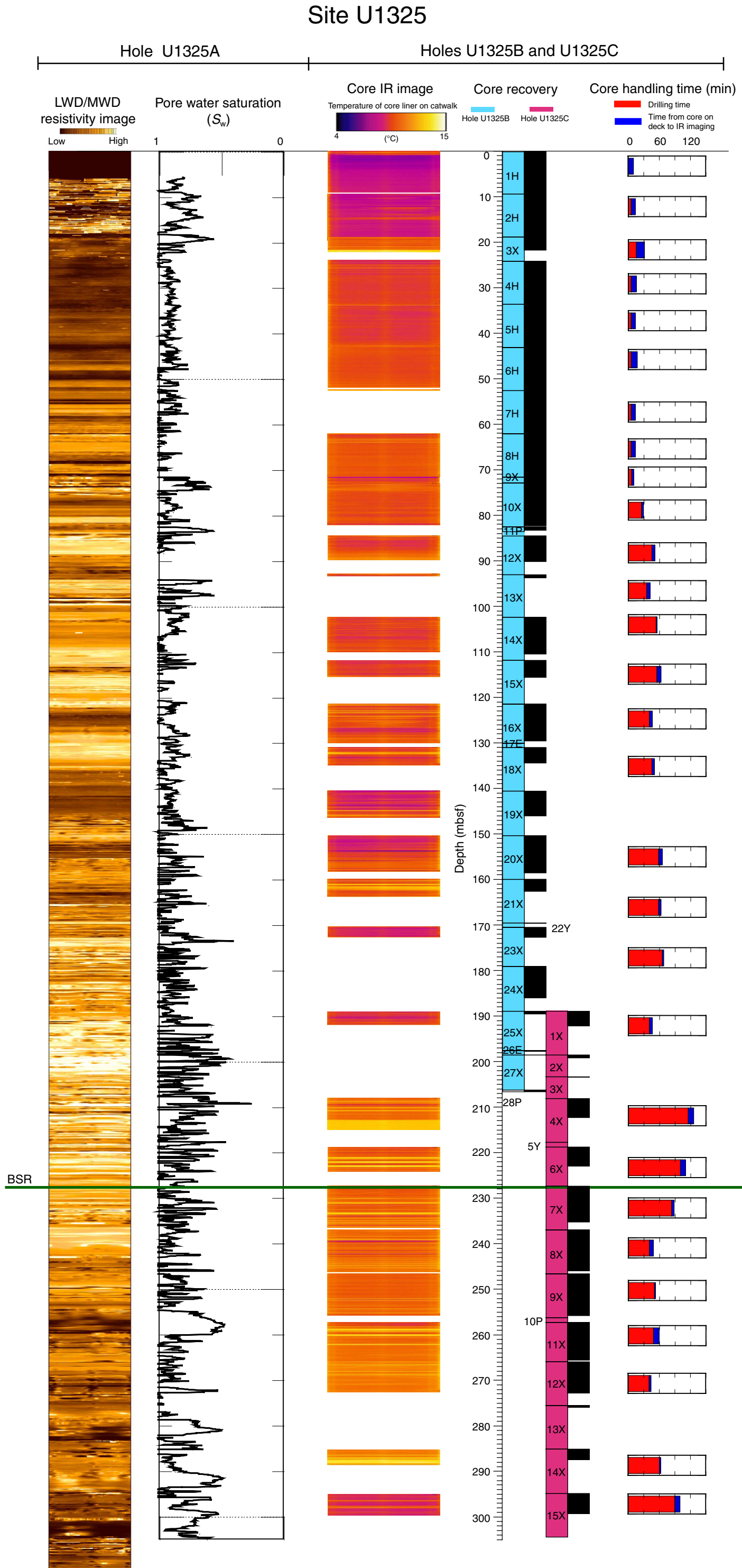
Site U1325, Figure F35. Combined infrared (IR) images of core liner temperature from Holes U1325B and U1325C compared to logging-while-drilling/measurement-while-drilling (LWD/MWD) resistivity and calculated pore water saturation from Hole U1325A. Core recovery and handling time are also shown. BSR = bottom-simulating reflector.
