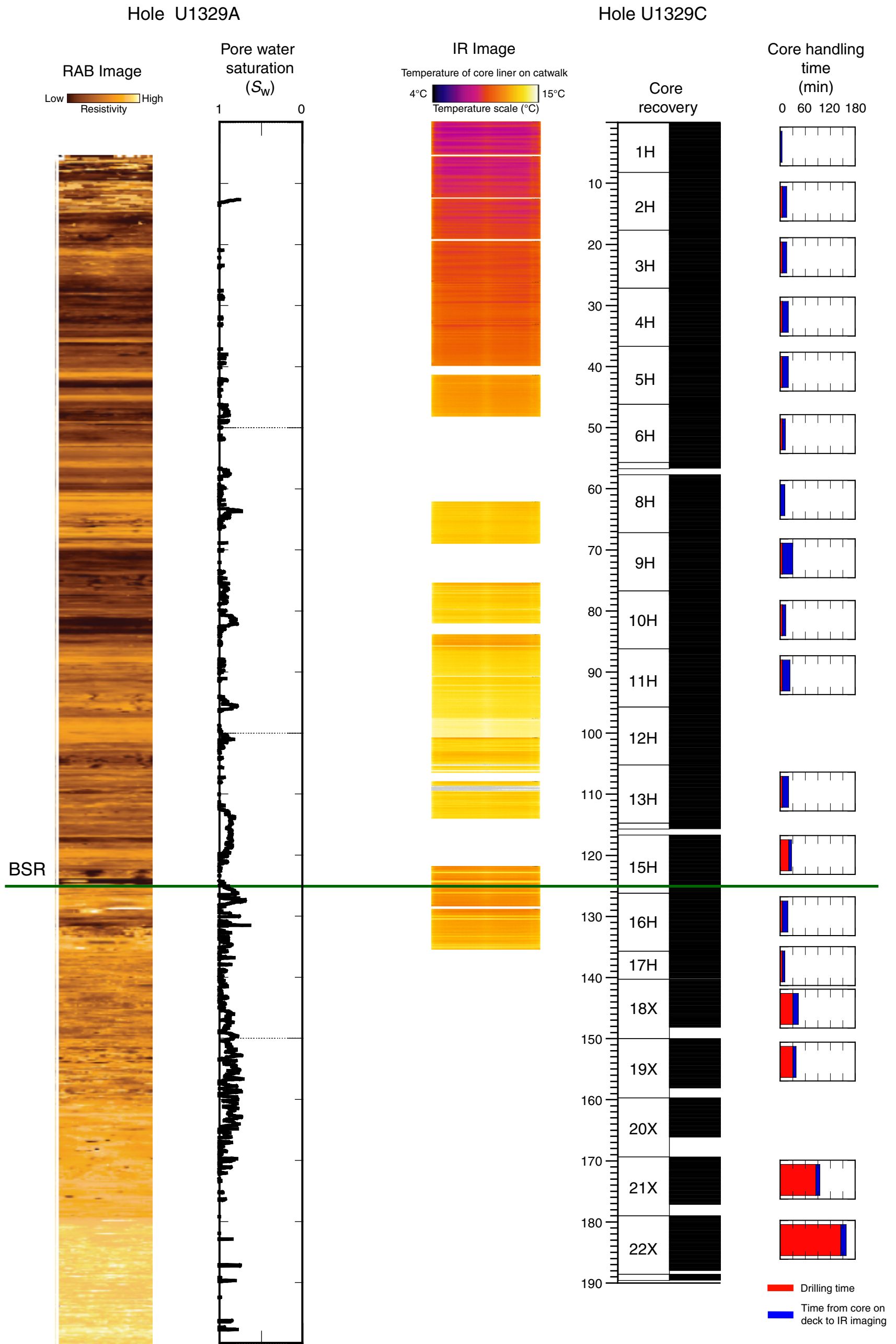
Site U1329, Figure F31. Combined infrared (IR) images of core liner temperature from Hole U1329C, compared to LWD resistivity and calculated pore water saturation from Hole U1329A. Core recovery and core handling time are also shown. RAB = resistivity-at-the-bit, BSR = bottom-simulating reflector.
