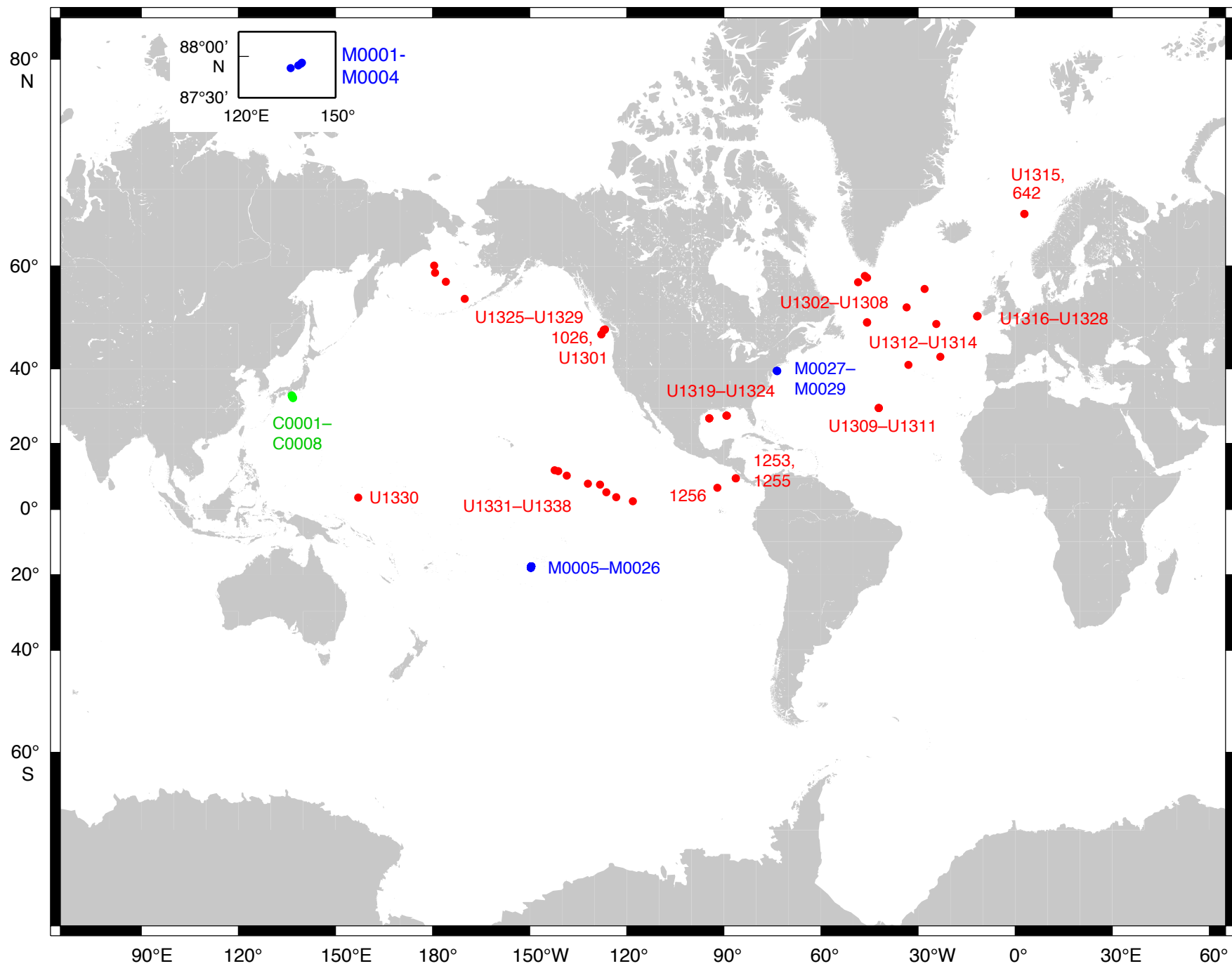
IODP Expeditions 301-316, 320-321, Sites C0001-C0008 (●), M0001-M0029 (●), U1301-U1338 (●)
