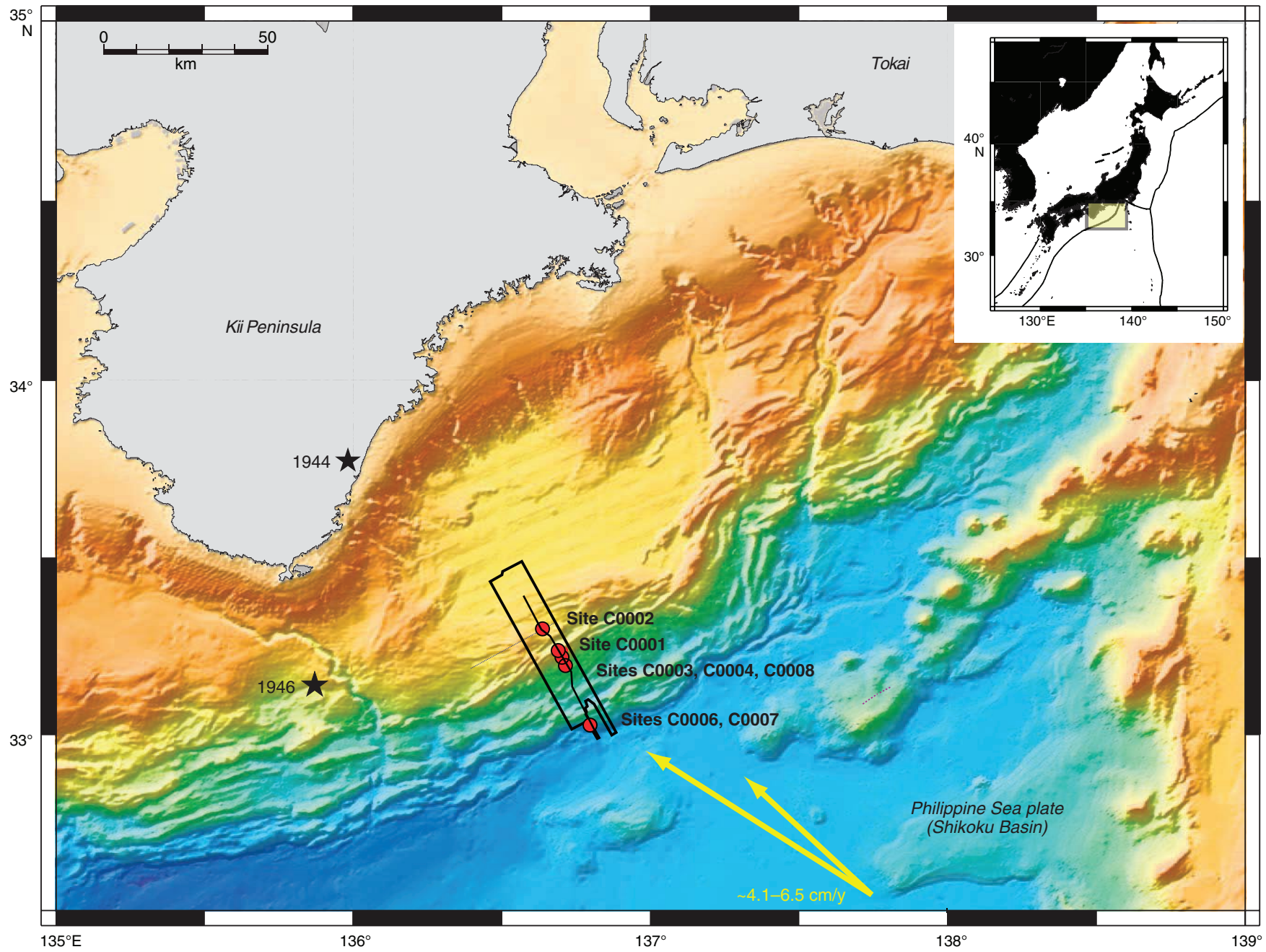
IODP Expedition 314/315/316 Site Map
