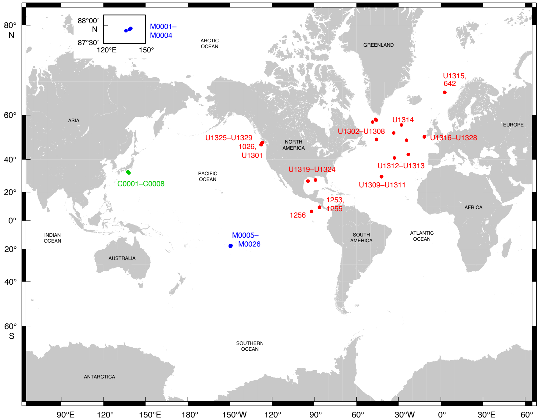
IODP Expeditions 301-312 & 314-316, Sites C0001-C0008 (●), M0001-M0026 (●), U1301-U1329 (●)
