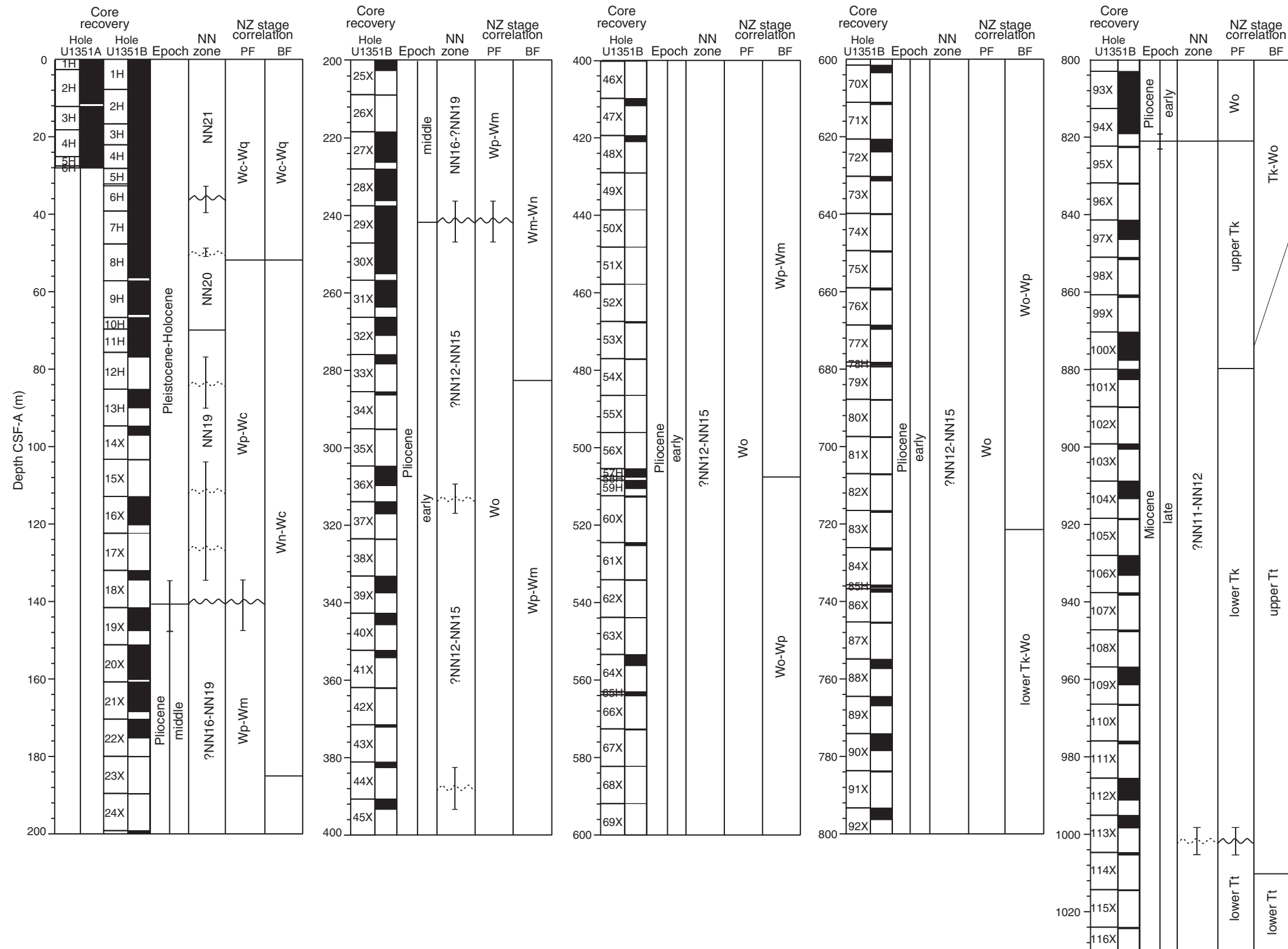
Figure F24. Core recovery, epochs, calcareous nannofossil (NN) zones, and New Zealand (NZ) stage correlation for planktonic foraminifers (PF) and benthic foraminifers (BF), Site U1351. Solid wavy lines = hiatuses between biozones, dashed wavy lines = hiatuses within biozones. See Figure F5 in the “Methods” chapter for NZ stage abbreviations.
