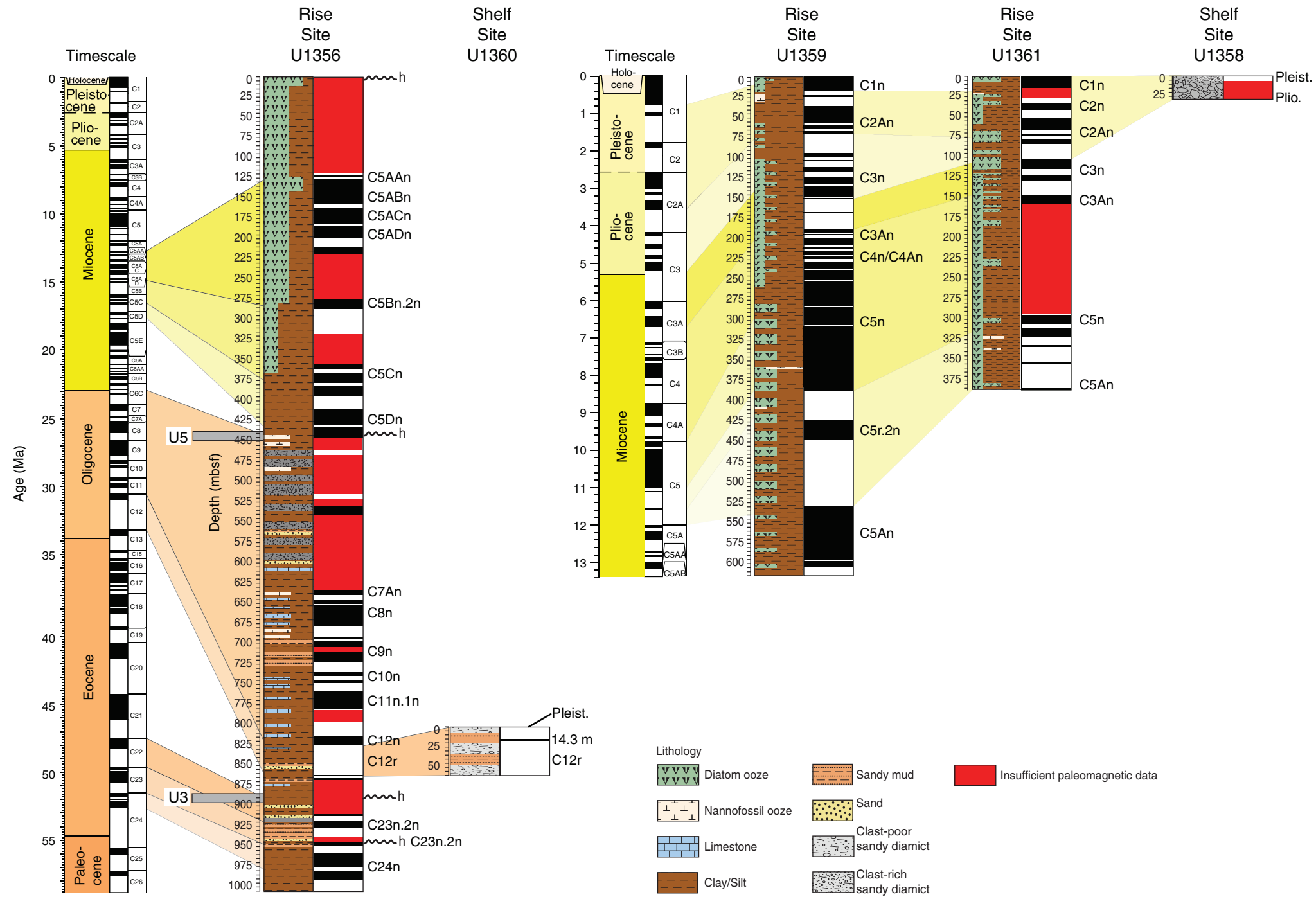
Figure F25. Chronostratigraphic framework for sites drilled during Expedition 318. Timescales are those of Gradstein et al. (2004).
