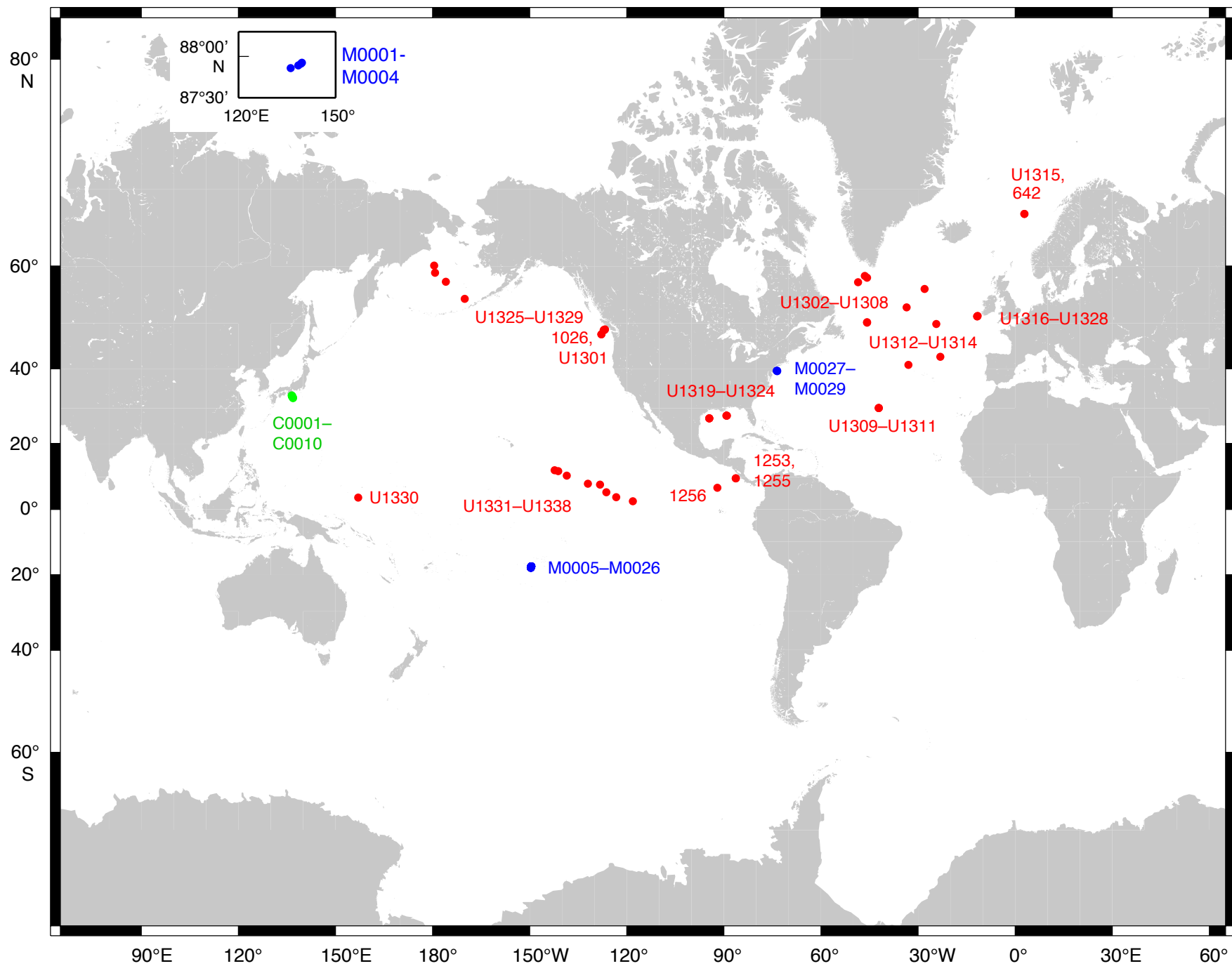
IODP Expeditions 301-316, 319-321, Sites C0001-C0010 (●), M0001-M0029 (●), U1301-U1338 (●)
