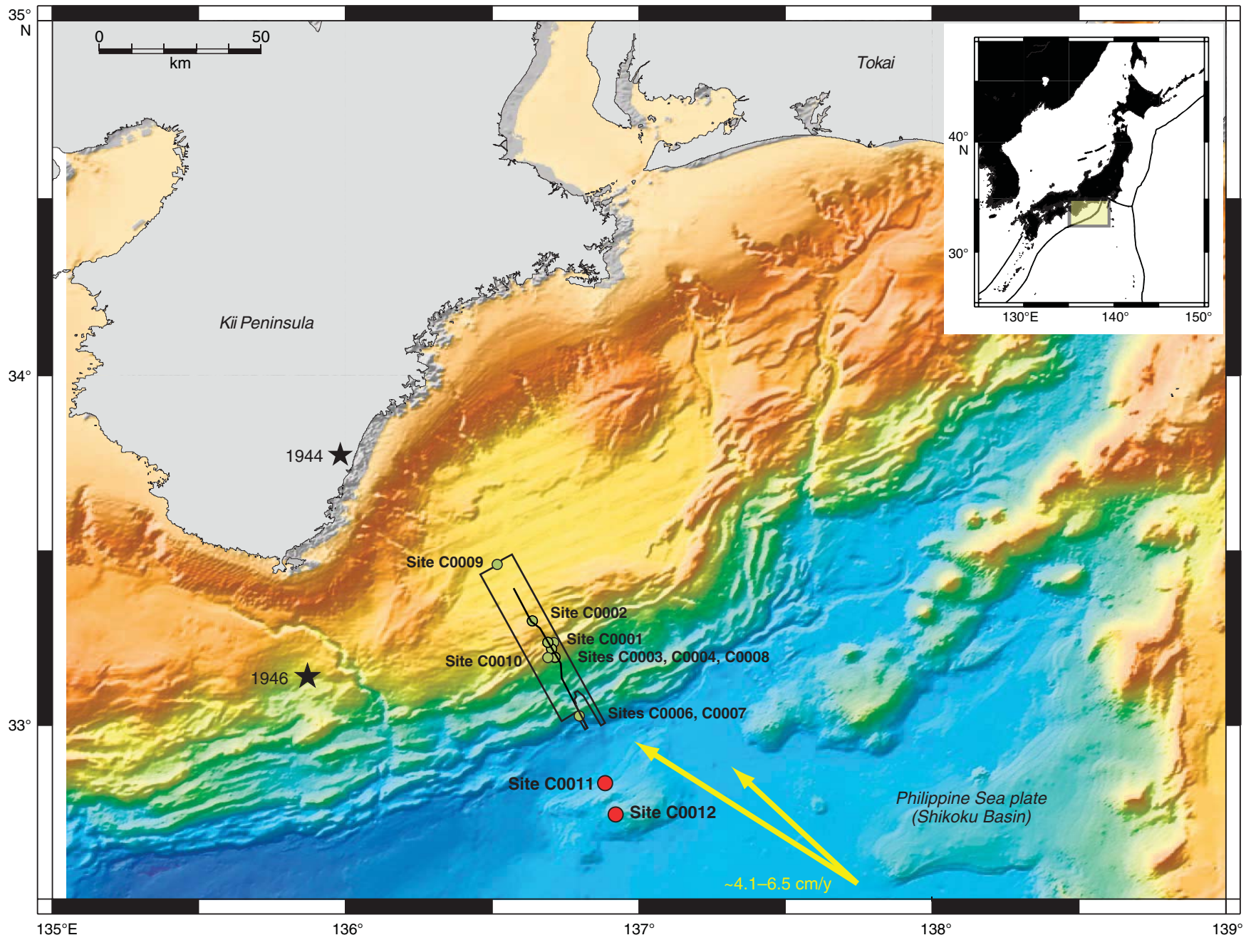
IODP Expedition 322 Site Map
