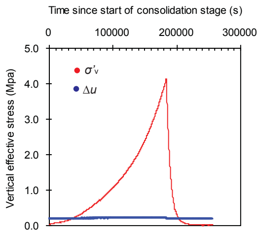
333-C0018A-11H-11, 0 cm
