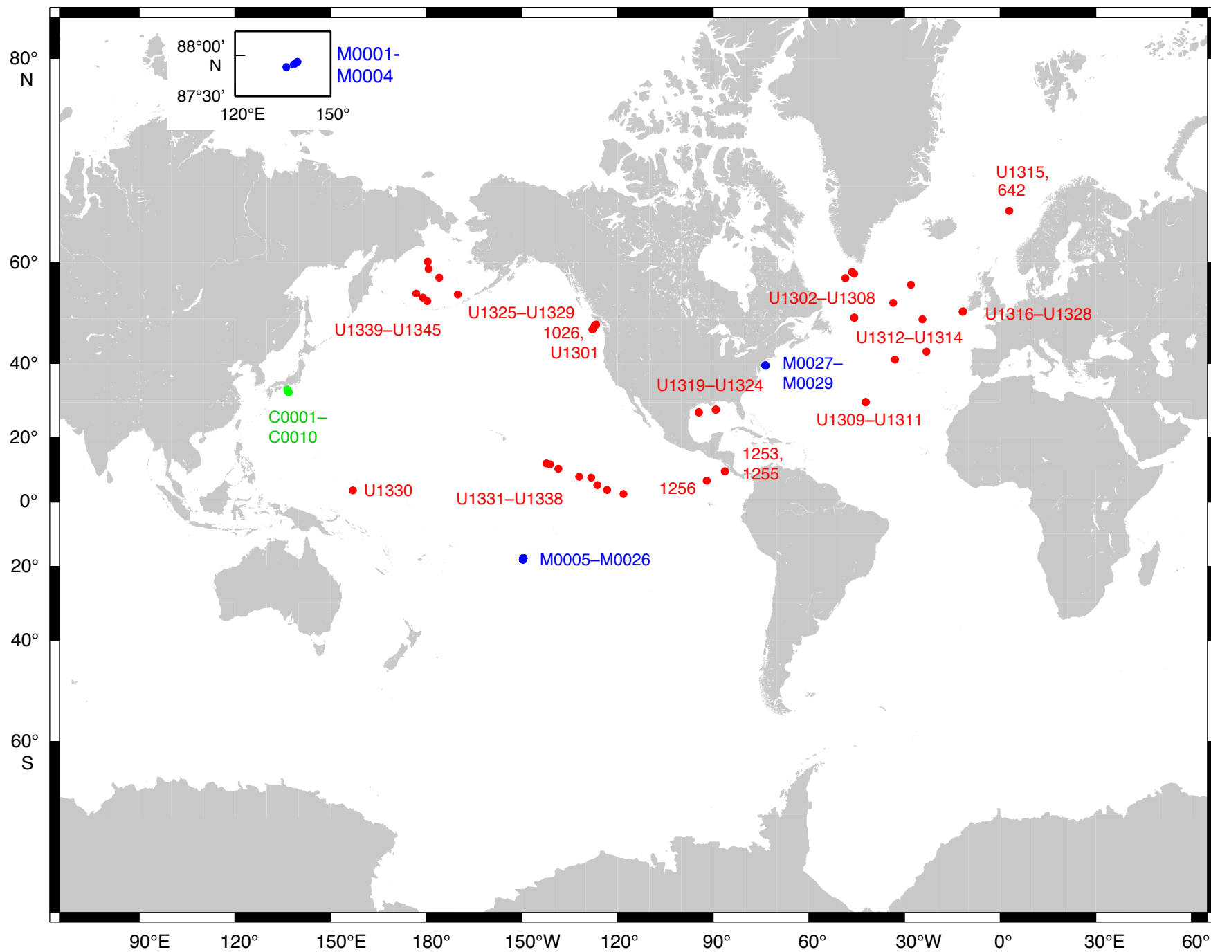
IODP Expeditions 301–316, 319–321, 323 Sites C0001–C0010 (●), M0001–M0029 (●), U1301–U1345 (●)
