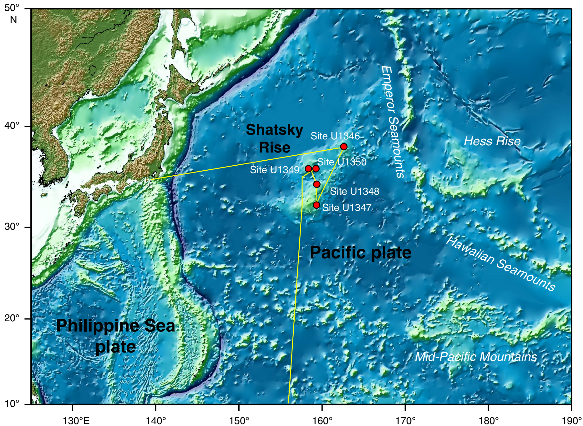
IODP Expedition 324 Site Map
