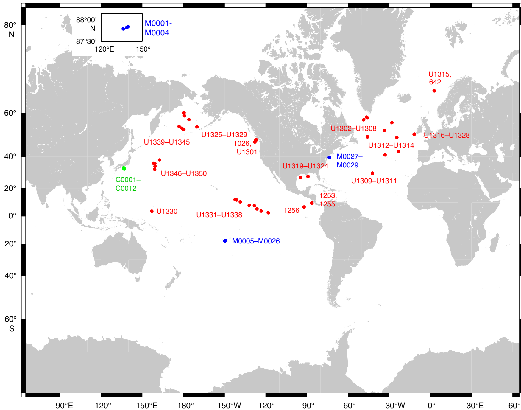
IODP Expeditions 301–316, 319–324, Sites C0001–C0012 (●), M0001–M0029 (●), U1301–U1350 (●)
