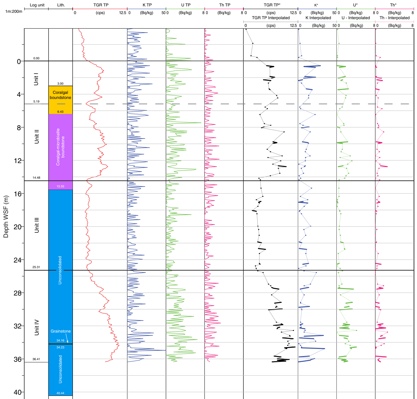
Transect HYD-01C, Figure F18. Composite showing all logging data collected in Hole M0031A. TGR = total gamma ray (raw), TP = through pipe. * = negative values removed.
