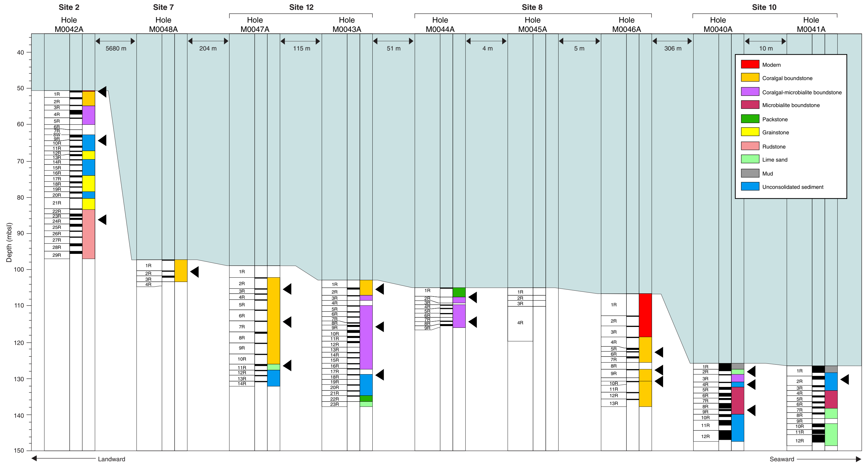
Figure F88. Transect summary showing recovery and main lithostratigraphic units interpreted for transect HYD-02A. Holes are plotted against present-day sea level (LAT taken from corrected EM300 multibeam bathymetry). Distances between holes are indicated on the diagram but are not drawn to horizontal scale.
