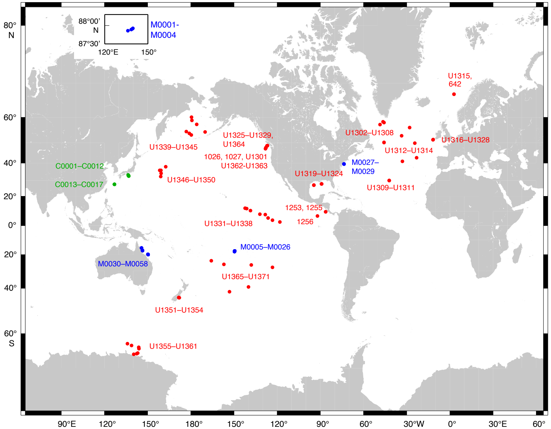
IODP Expeditions 301-329, 331, Sites C0001-C0017 (●), M0001-M0058 (●), U1301-U1371 (●)
