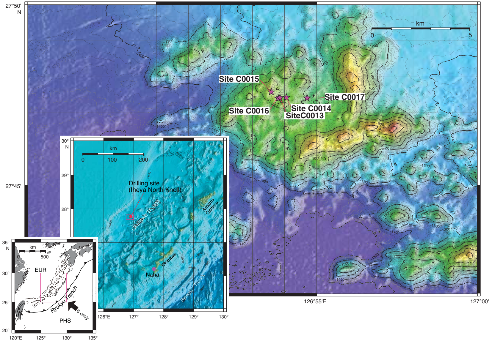
IODP Expedition 331 Site Map
