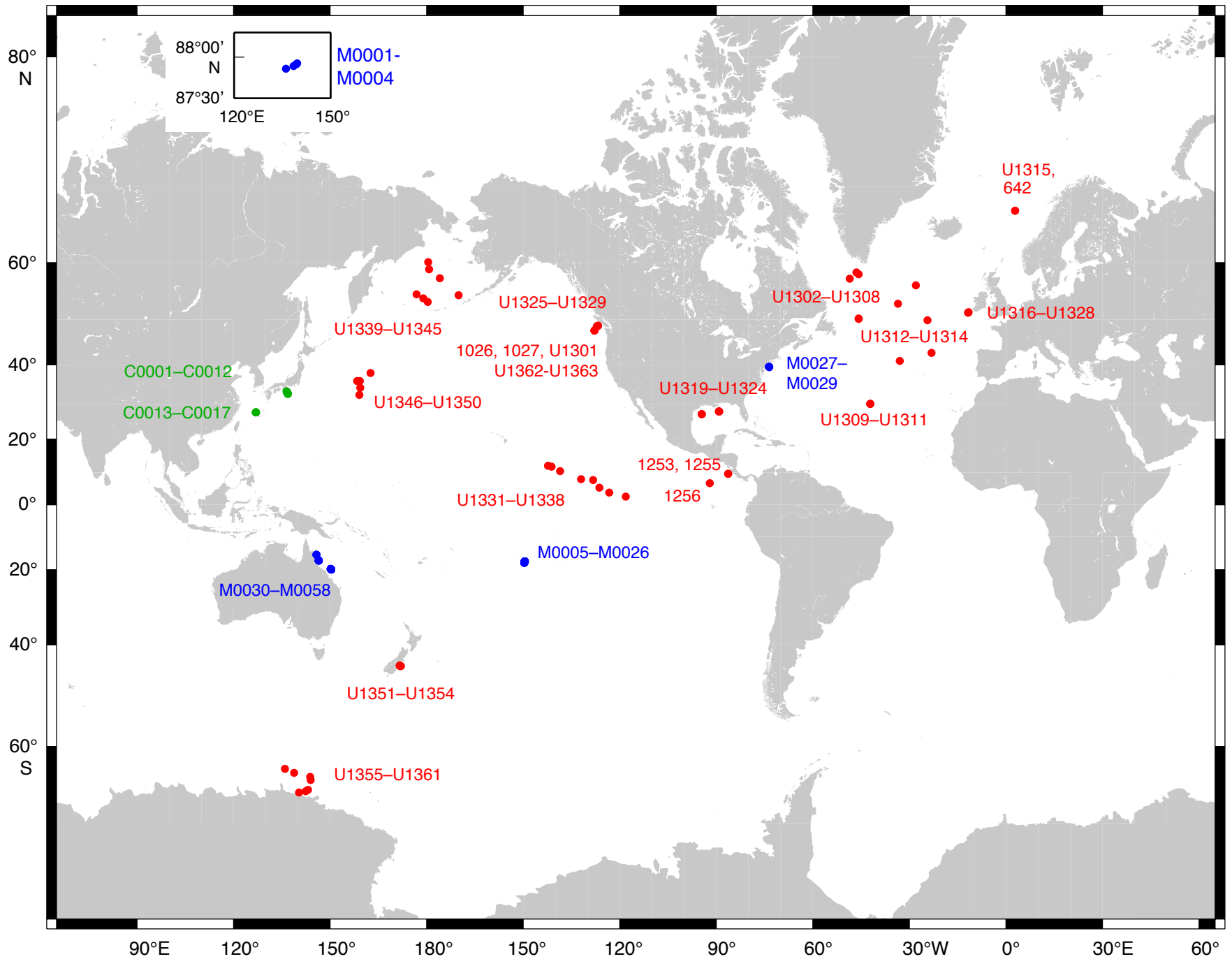
IODP Expeditions 301–327, 331, Sites C0001–C0017 (●), M0001–M0058 (●), U1301–U1363 (●)
