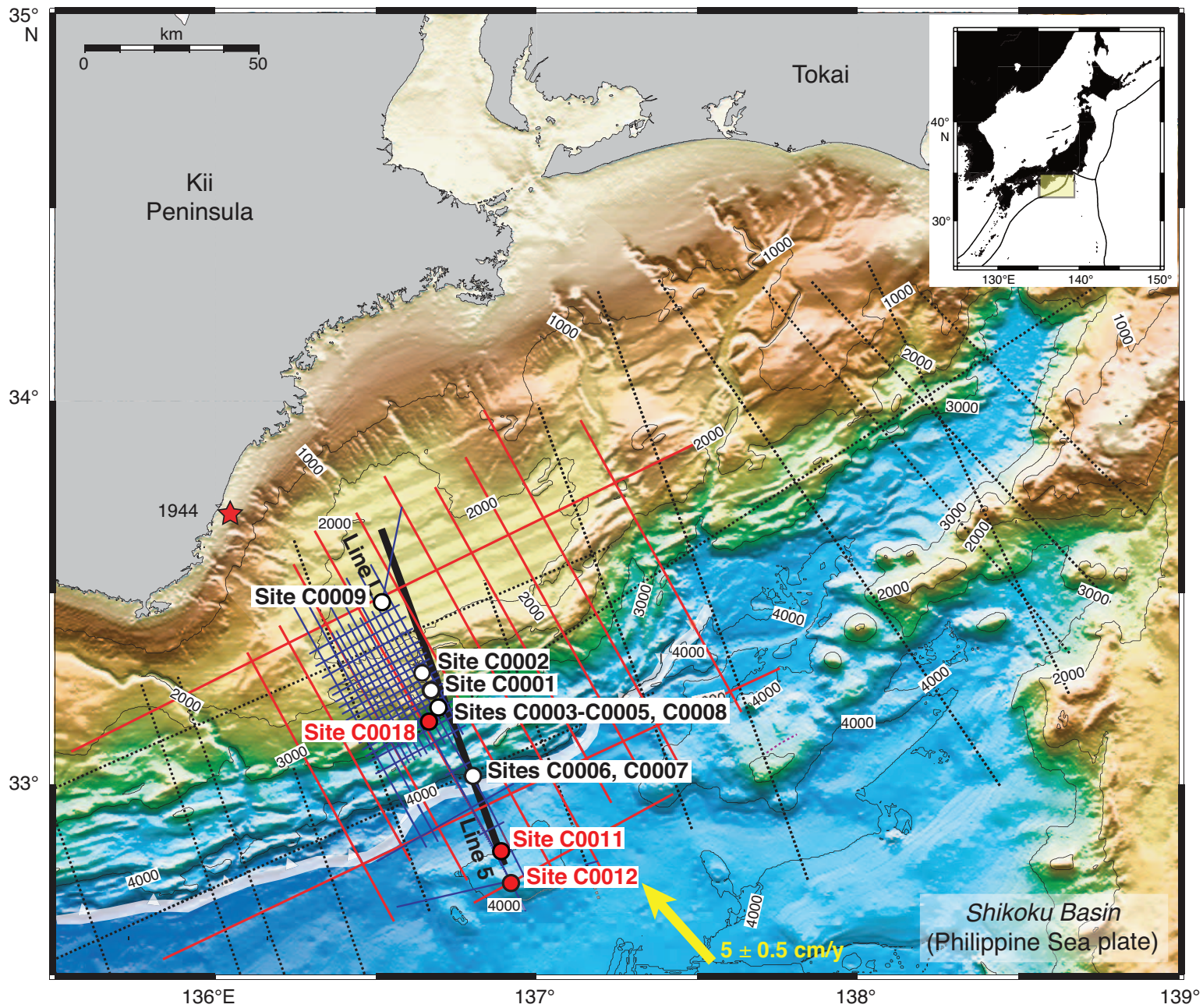
IODP Expedition 333 Site Map
