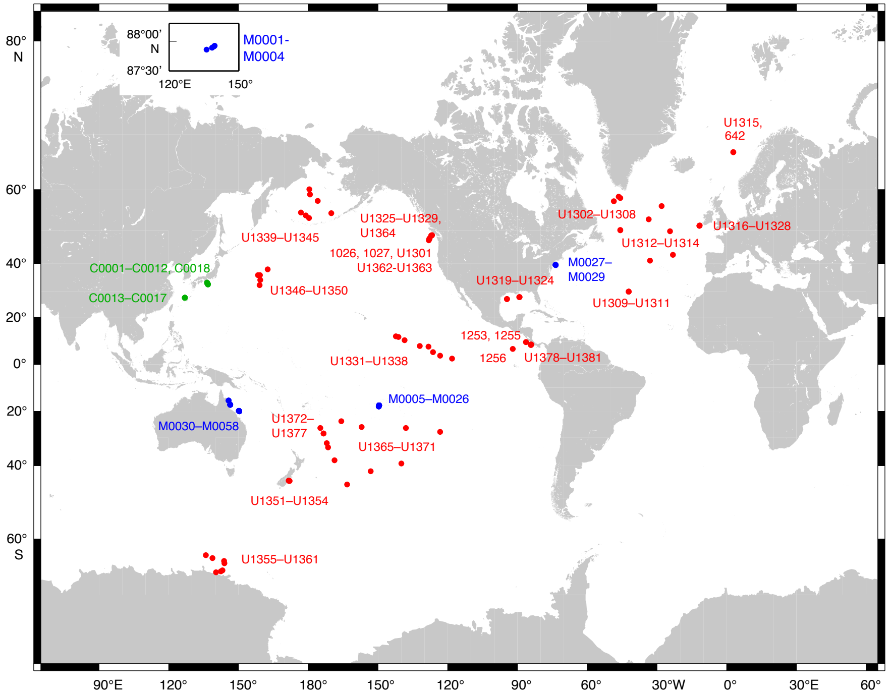
IODP Expeditions 301-334, Sites C0001-C0018 (●), M0001-M0058 (●), U1301-U1381 (●)
