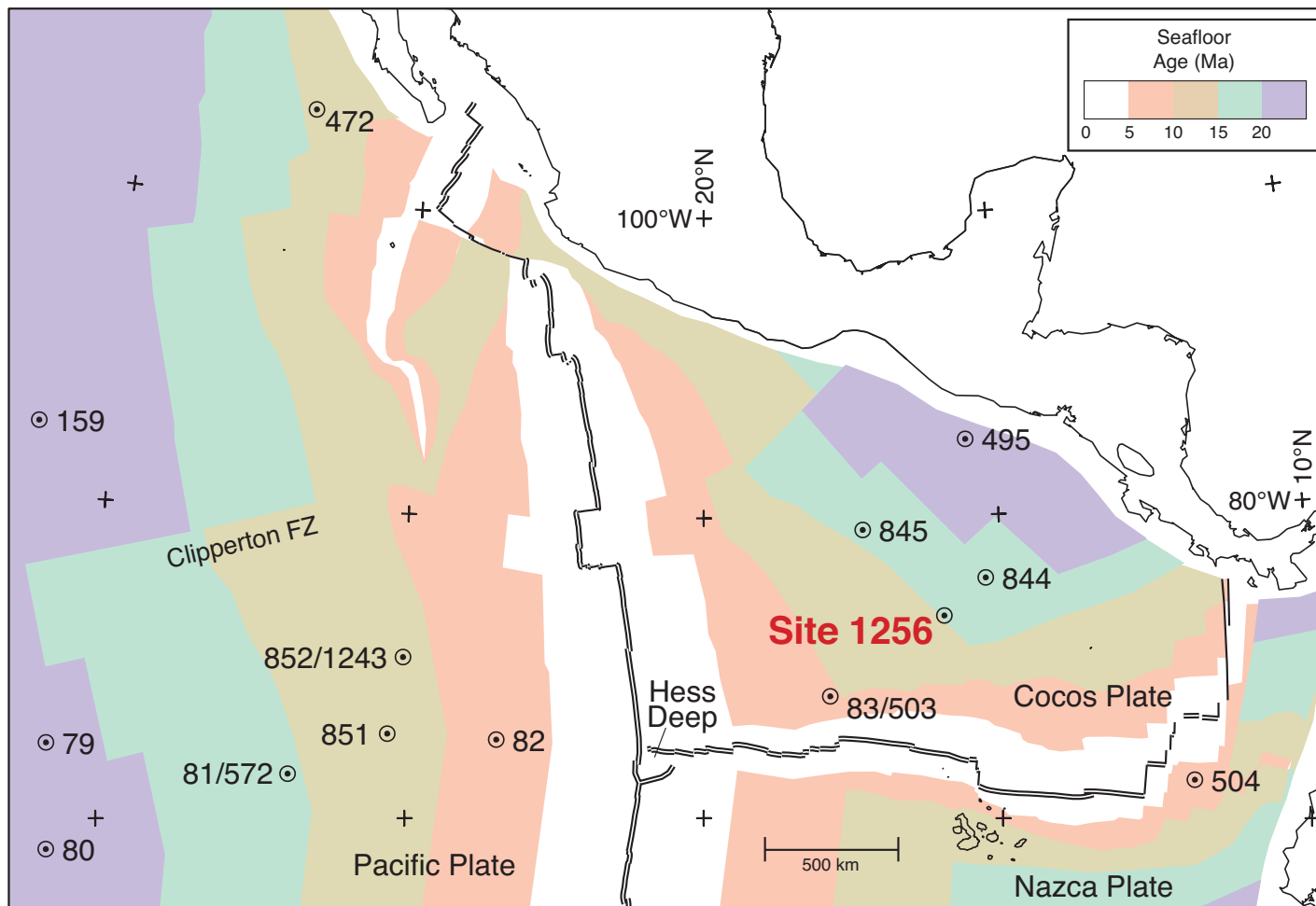
IODP Expedition 335 Site Map
