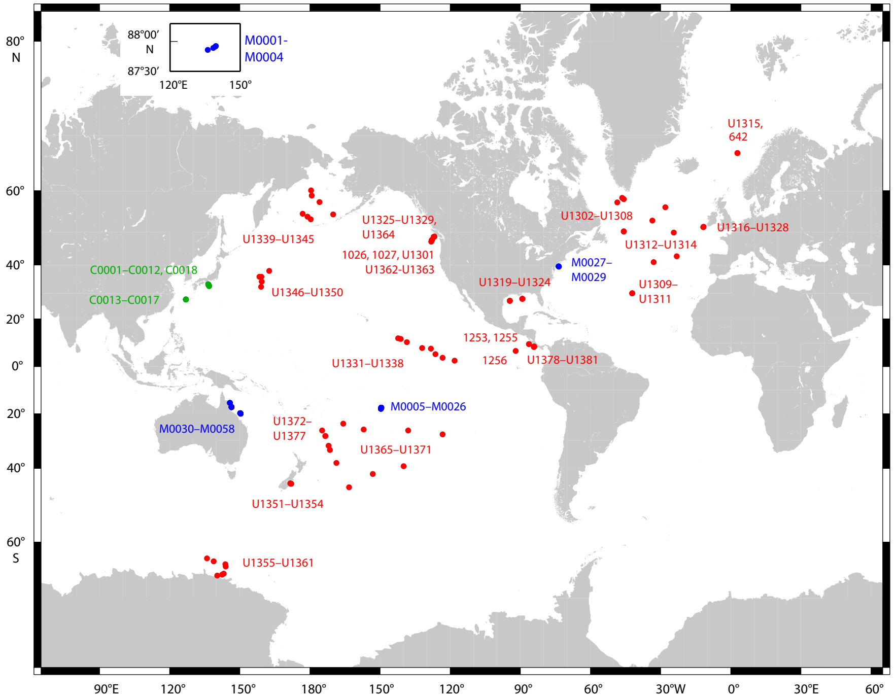
IODP Expeditions 301-335, Sites C0001-C0018 (●), M0001-M0058 (●), U1301-U1384 (●)
